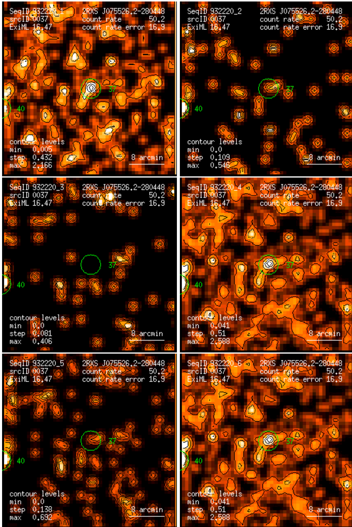
Figure 37: RASS 932220: detection 0037: band rate images, Gaussian filter: (1) PSPC channels 11 – 41, (2) 52 – 90, (3) 91 – 201, (4) 11 – 235, (5) 52 – 201, (6) 11 – 201. Broad band rates in counts/ks. Band rate contour levels in counts/ks/arcmin 2 .
