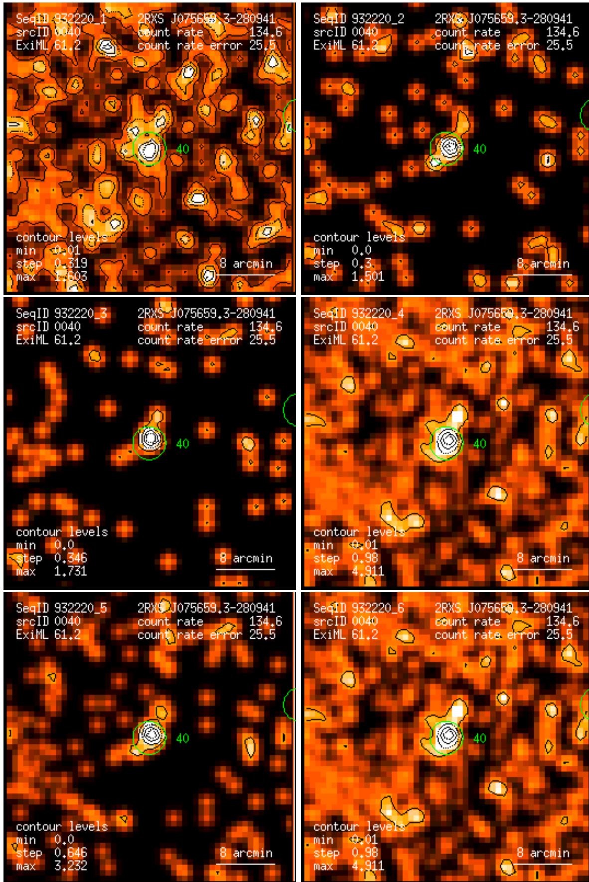
Figure 40: RASS 932220: detection 0040: band rate images, Gaussian filter: (1) PSPC channels 11 – 41, (2) 52 – 90, (3) 91 – 201, (4) 11 – 235, (5) 52 – 201, (6) 11 – 201. Broad band rates in counts/ks. Band rate contour levels in counts/ks/arcmin 2 .
