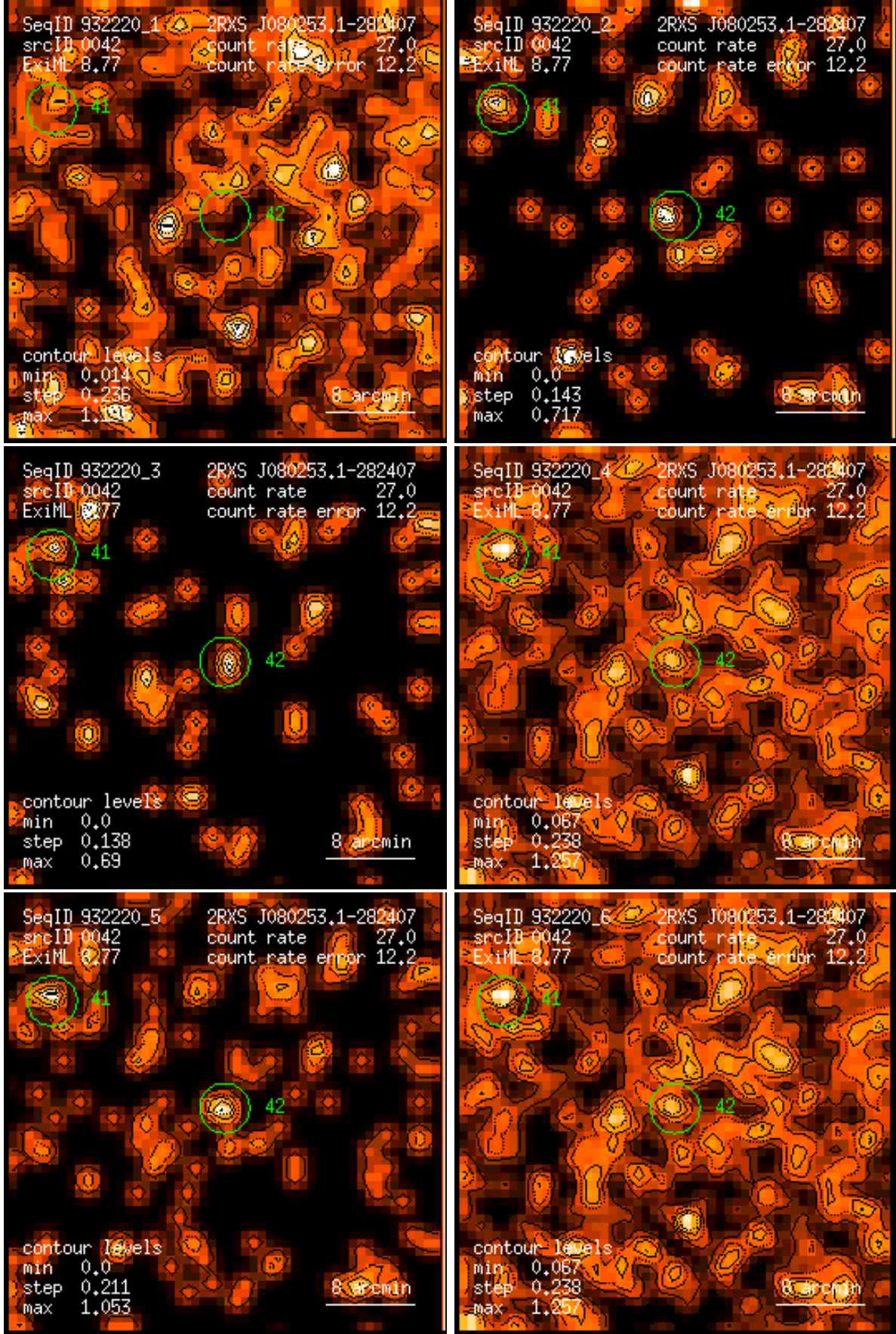
Figure 42: RASS 932220: detection 0042: band rate images, Gaussian filter: (1) PSPC channels 11 – 41, (2) 52 – 90, (3) 91 – 201, (4) 11 – 235, (5) 52 – 201, (6) 11 – 201. Broad band rates in counts/ks. Band rate contour levels in counts/ks/arcmin 2 .
