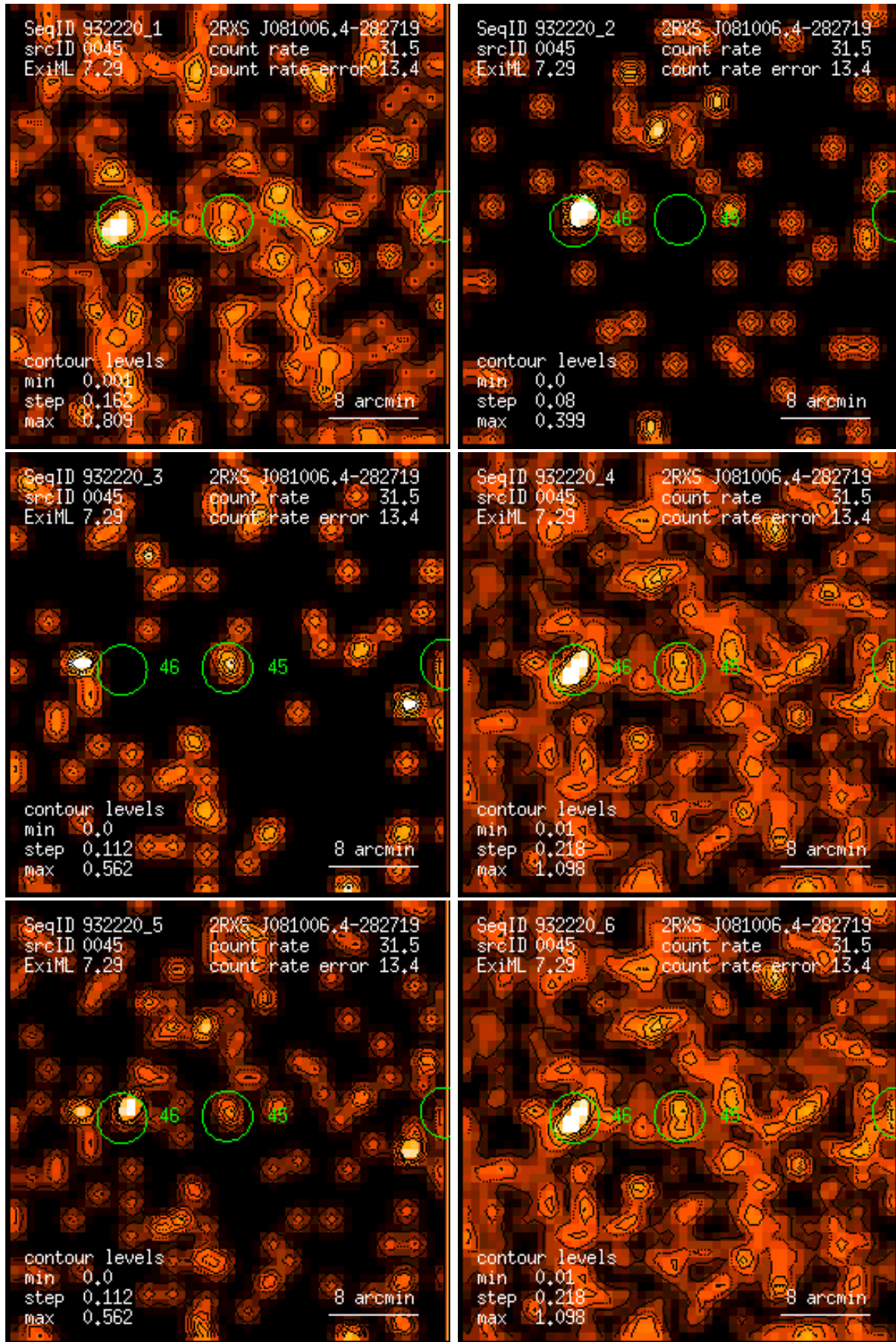
Figure 45: RASS 932220: detection 0045: band rate images, Gaussian filter: (1) PSPC channels 11 – 41, (2) 52 – 90, (3) 91 – 201, (4) 11 – 235, (5) 52 – 201, (6) 11 – 201. Broad band rates in counts/ks. Band rate contour levels in counts/ks/arcmin 2 .
