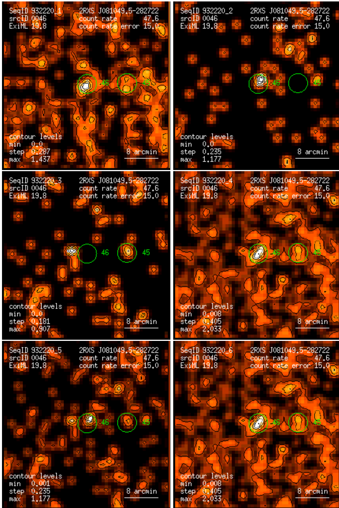
Figure 46: RASS 932220: detection 0046: band rate images, Gaussian filter: (1) PSPC channels 11 – 41, (2) 52 – 90, (3) 91 – 201, (4) 11 – 235, (5) 52 – 201, (6) 11 – 201. Broad band rates in counts/ks. Band rate contour levels in counts/ks/arcmin 2 .
