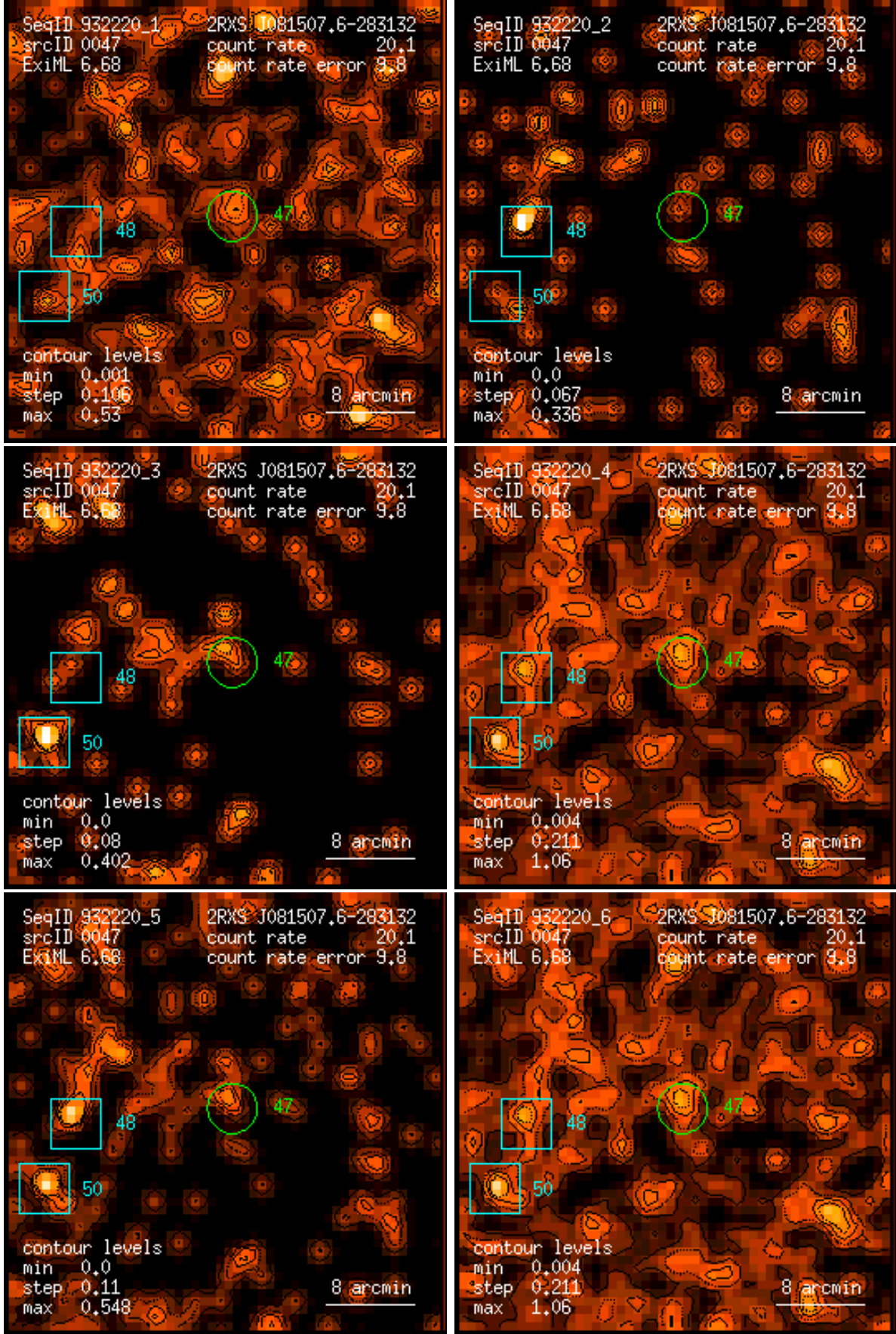
Figure 47: RASS 932220: detection 0047: band rate images, Gaussian filter: (1) PSPC channels 11 – 41, (2) 52 – 90, (3) 91 – 201, (4) 11 – 235, (5) 52 – 201, (6) 11 – 201. Broad band rates in counts/ks. Band rate contour levels in counts/ks/arcmin 2 .
