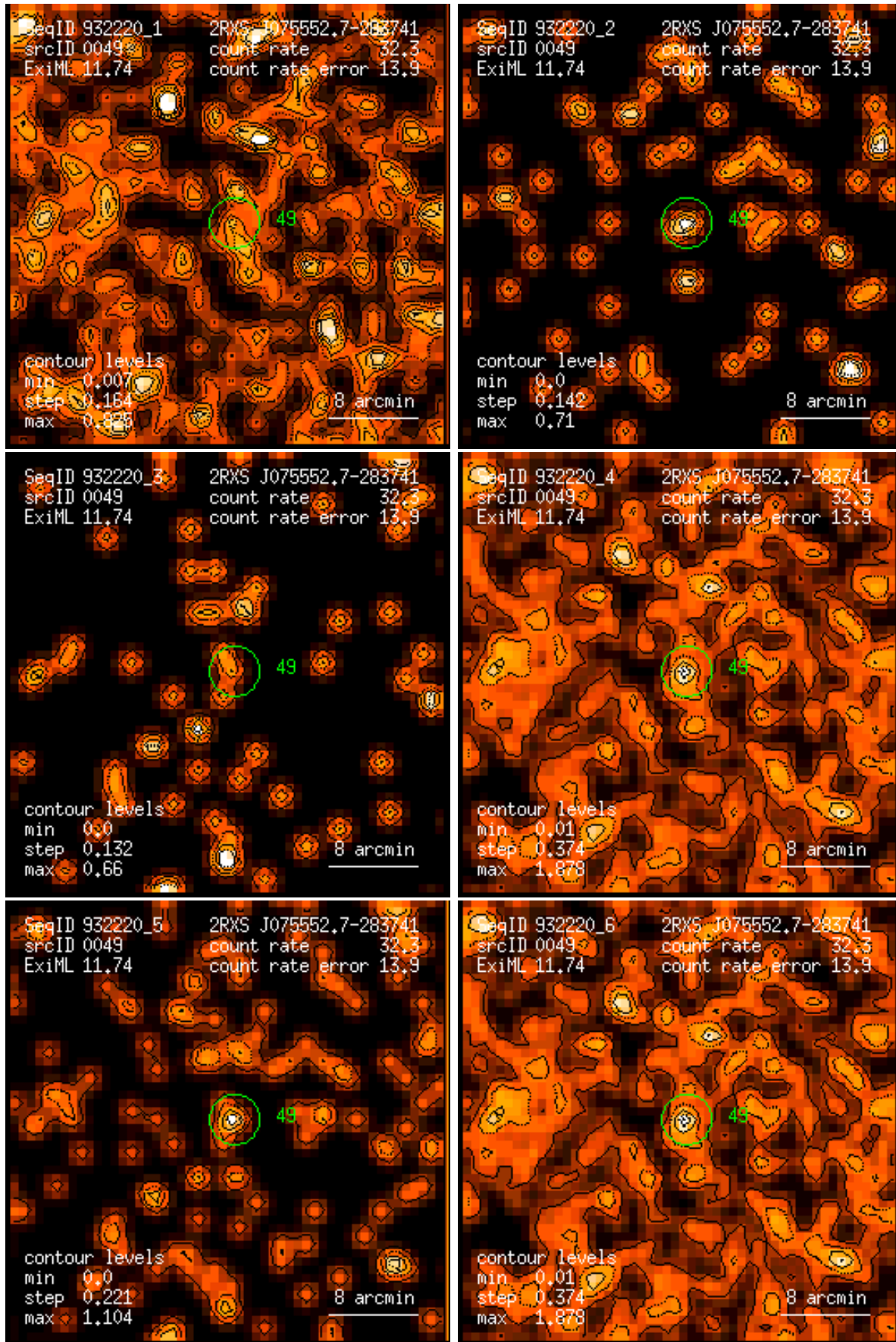
Figure 49: RASS 932220: detection 0049: band rate images, Gaussian filter: (1) PSPC channels 11 – 41, (2) 52 – 90, (3) 91 – 201, (4) 11 – 235, (5) 52 – 201, (6) 11 – 201. Broad band rates in counts/ks. Band rate contour levels in counts/ks/arcmin 2 .
