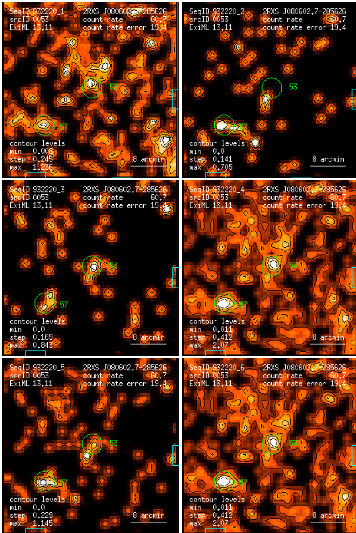
Figure 53: RASS 932220: detection 0053: band rate images, Gaussian filter: (1) PSPC channels 11 – 41, (2) 52 – 90, (3) 91 – 201, (4) 11 – 235, (5) 52 – 201, (6) 11 – 201. Broad band rates in counts/ks. Band rate contour levels in counts/ks/arcmin 2 .
