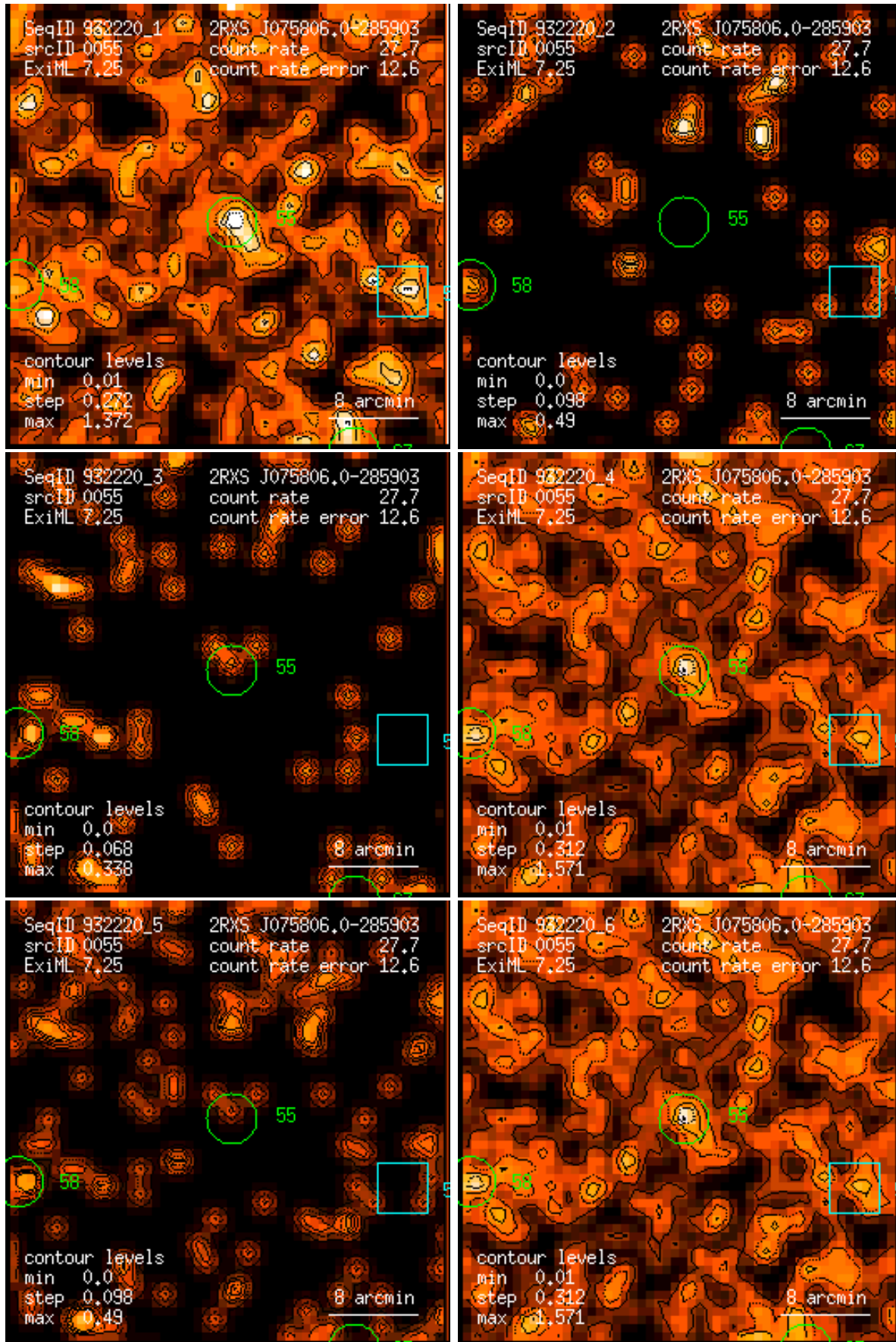
Figure 55: RASS 932220: detection 0055: band rate images, Gaussian filter: (1) PSPC channels 11 – 41, (2) 52 – 90, (3) 91 – 201, (4) 11 – 235, (5) 52 – 201, (6) 11 – 201. Broad band rates in counts/ks. Band rate contour levels in counts/ks/arcmin 2 .
