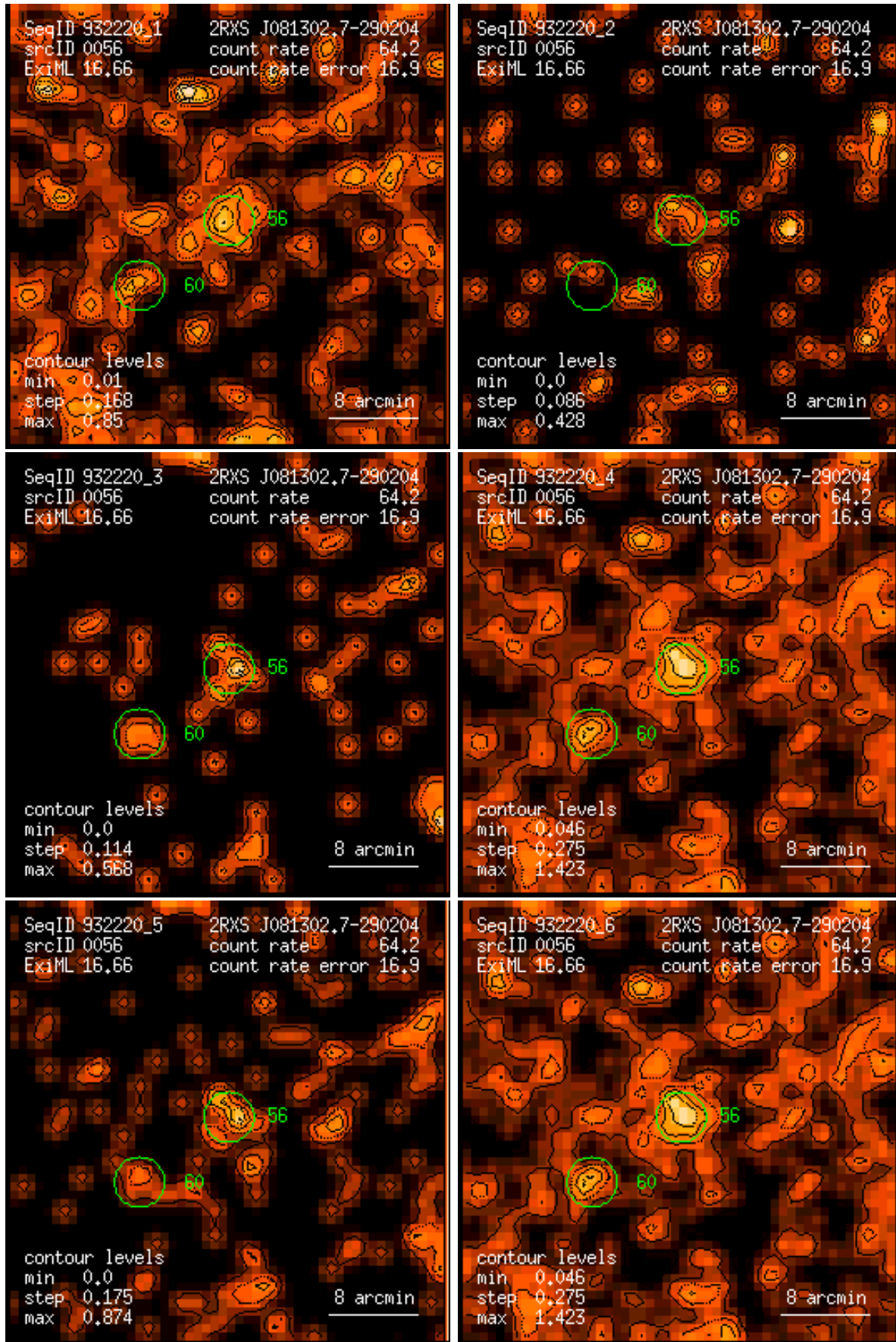
Figure 56: RASS 932220: detection 0056: band rate images, Gaussian filter: (1) PSPC channels 11 – 41, (2) 52 – 90, (3) 91 – 201, (4) 11 – 235, (5) 52 – 201, (6) 11 – 201. Broad band rates in counts/ks. Band rate contour levels in counts/ks/arcmin 2 .
