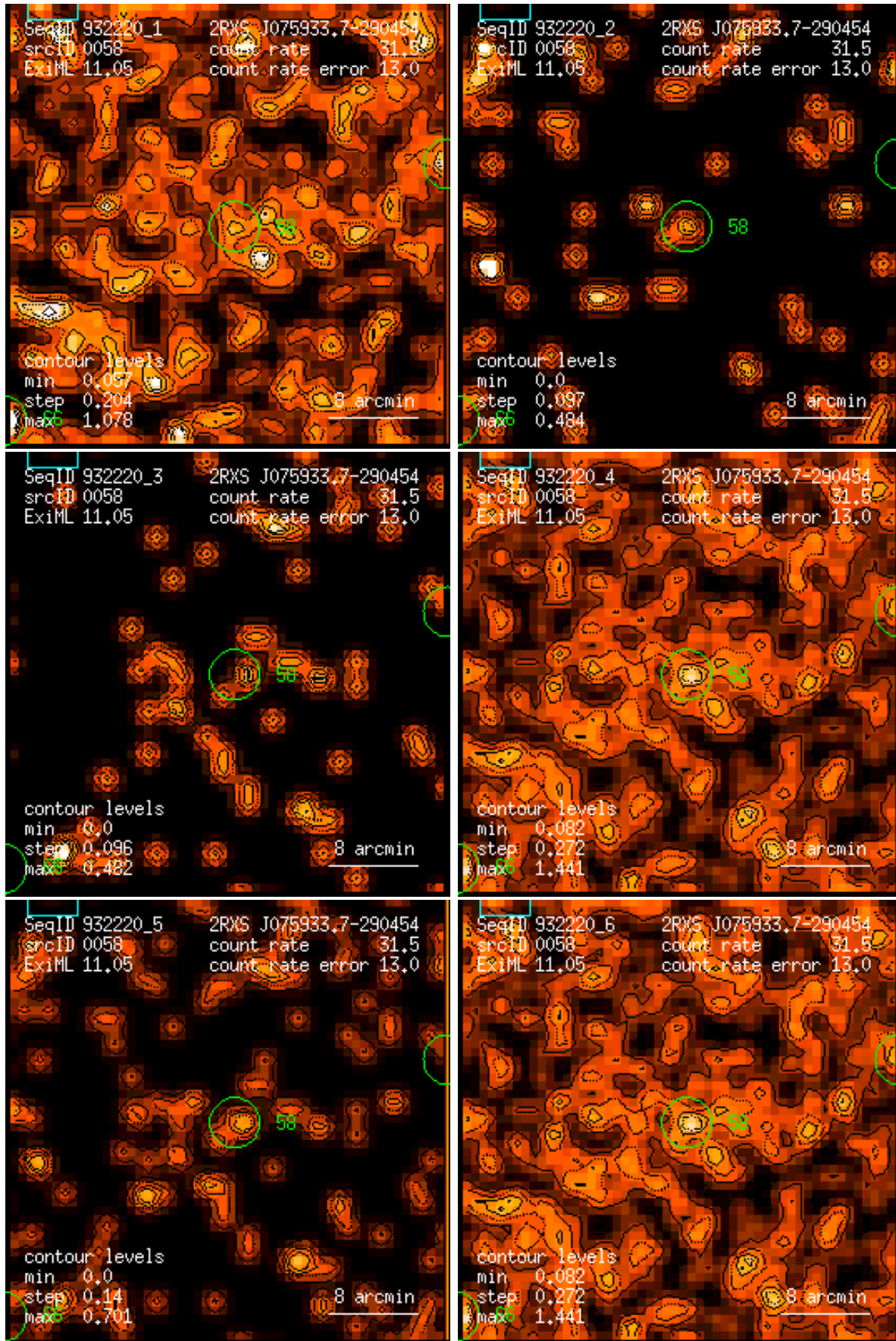
Figure 58: RASS 932220: detection 0058: band rate images, Gaussian filter: (1) PSPC channels 11 – 41, (2) 52 – 90, (3) 91 – 201, (4) 11 – 235, (5) 52 – 201, (6) 11 – 201. Broad band rates in counts/ks. Band rate contour levels in counts/ks/arcmin 2 .
