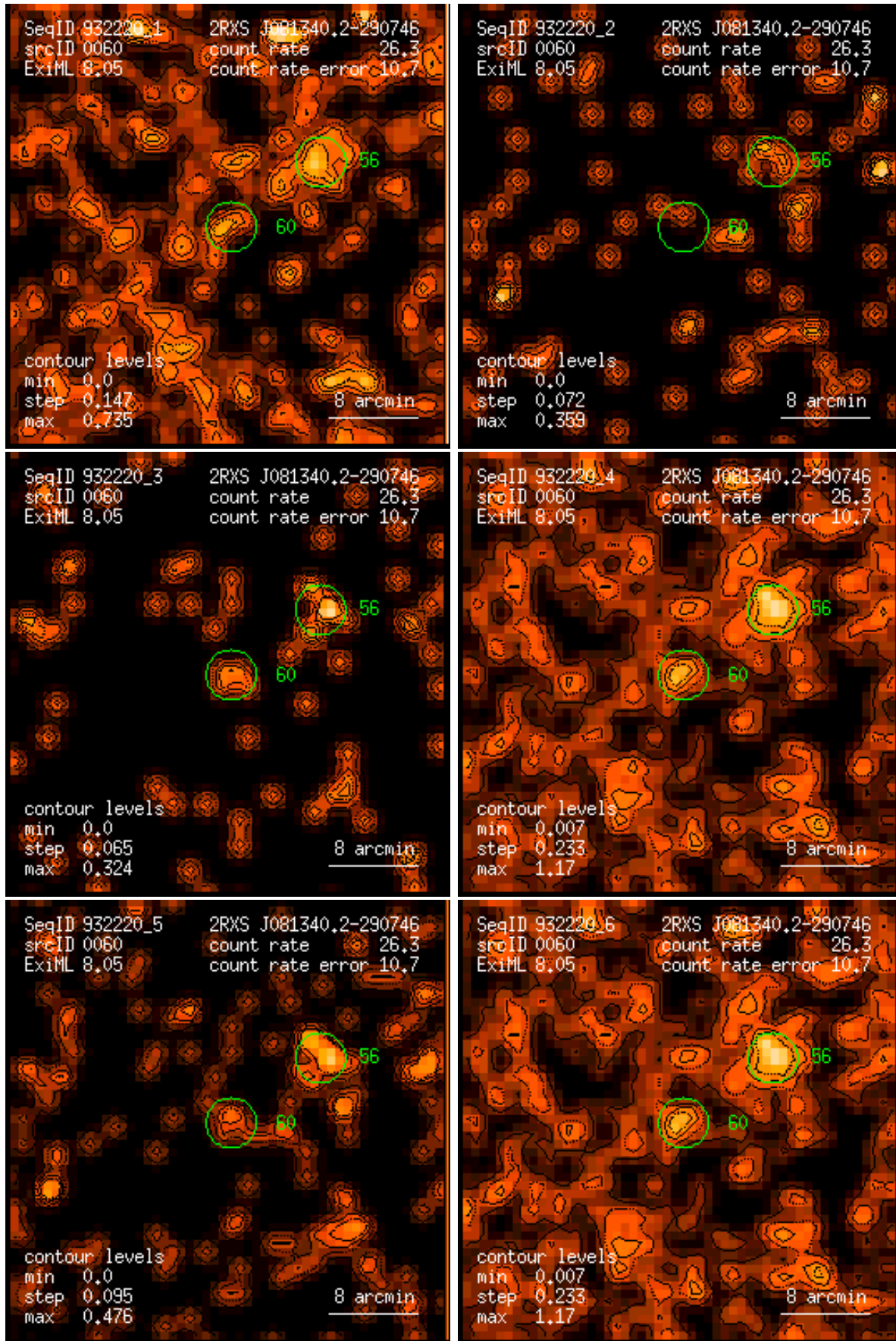
Figure 60: RASS 932220: detection 0060: band rate images, Gaussian filter: (1) PSPC channels 11 – 41, (2) 52 – 90, (3) 91 – 201, (4) 11 – 235, (5) 52 – 201, (6) 11 – 201. Broad band rates in counts/ks. Band rate contour levels in counts/ks/arcmin 2 .
