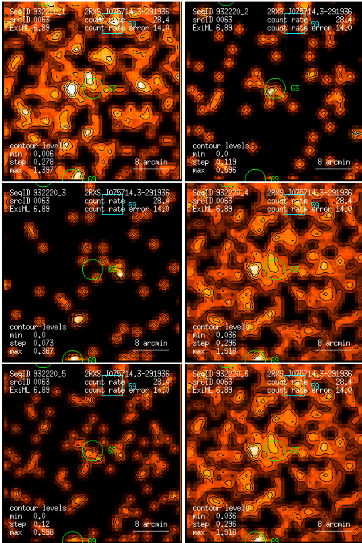
Figure 63: RASS 932220: detection 0063: band rate images, Gaussian filter: (1) PSPC channels 11 – 41, (2) 52 – 90, (3) 91 – 201, (4) 11 – 235, (5) 52 – 201, (6) 11 – 201. Broad band rates in counts/ks. Band rate contour levels in counts/ks/arcmin 2 .
