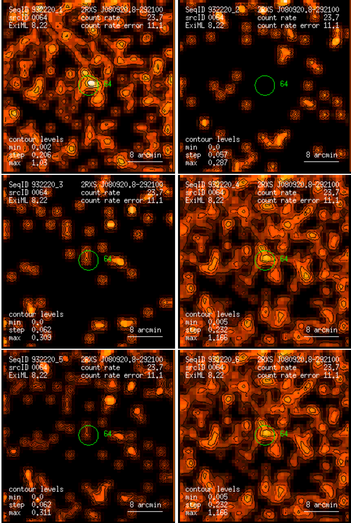
Figure 64: RASS 932220: detection 0064: band rate images, Gaussian filter: (1) PSPC channels 11 – 41, (2) 52 – 90, (3) 91 – 201, (4) 11 – 235, (5) 52 – 201, (6) 11 – 201. Broad band rates in counts/ks. Band rate contour levels in counts/ks/arcmin 2 .
