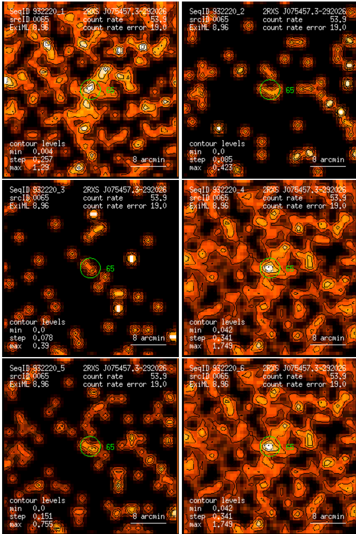
Figure 65: RASS 932220: detection 0065: band rate images, Gaussian filter: (1) PSPC channels 11 – 41, (2) 52 – 90, (3) 91 – 201, (4) 11 – 235, (5) 52 – 201, (6) 11 – 201. Broad band rates in counts/ks. Band rate contour levels in counts/ks/arcmin 2 .
