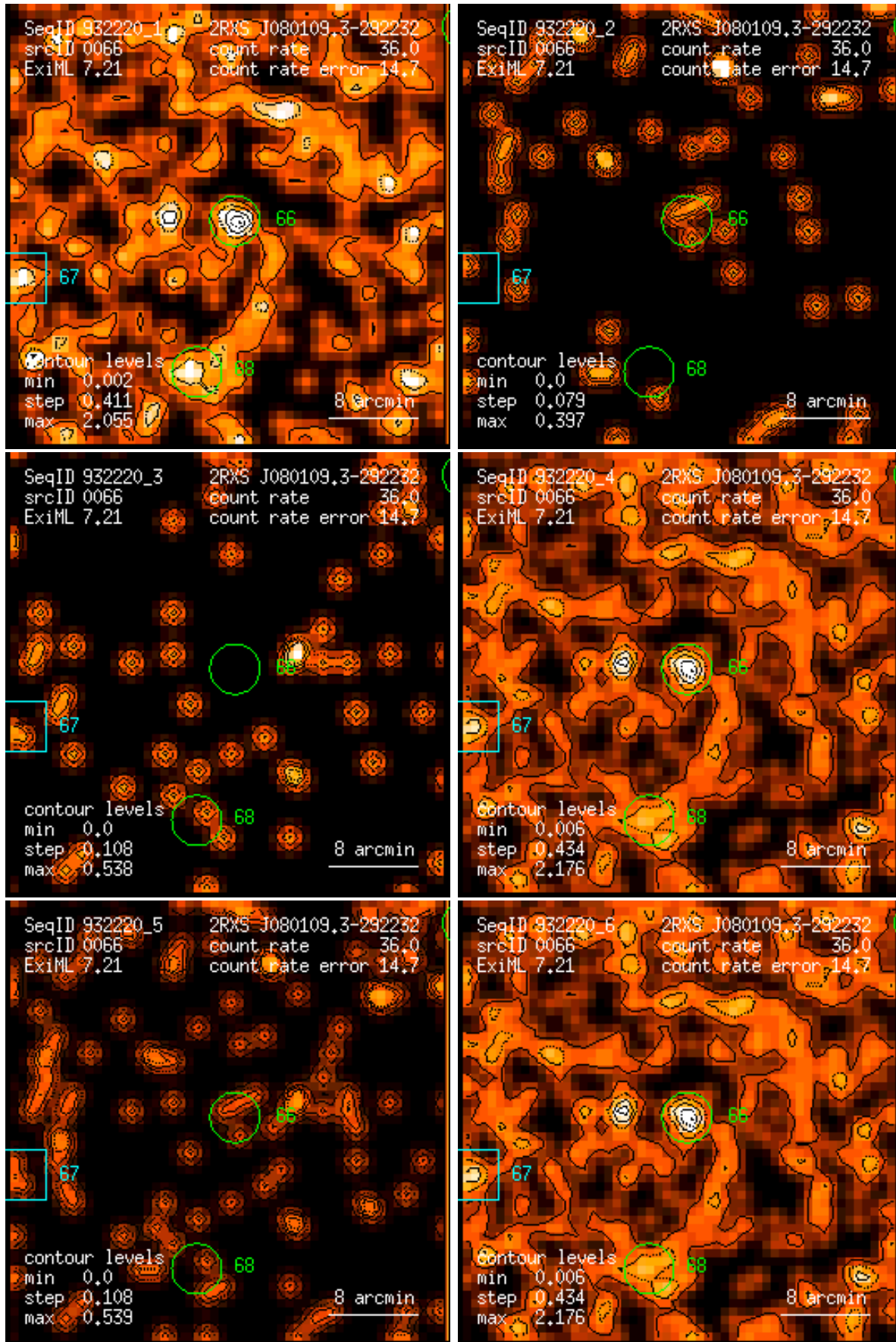
Figure 66: RASS 932220: detection 0066: band rate images, Gaussian filter: (1) PSPC channels 11 – 41, (2) 52 – 90, (3) 91 – 201, (4) 11 – 235, (5) 52 – 201, (6) 11 – 201. Broad band rates in counts/ks. Band rate contour levels in counts/ks/arcmin 2 .
