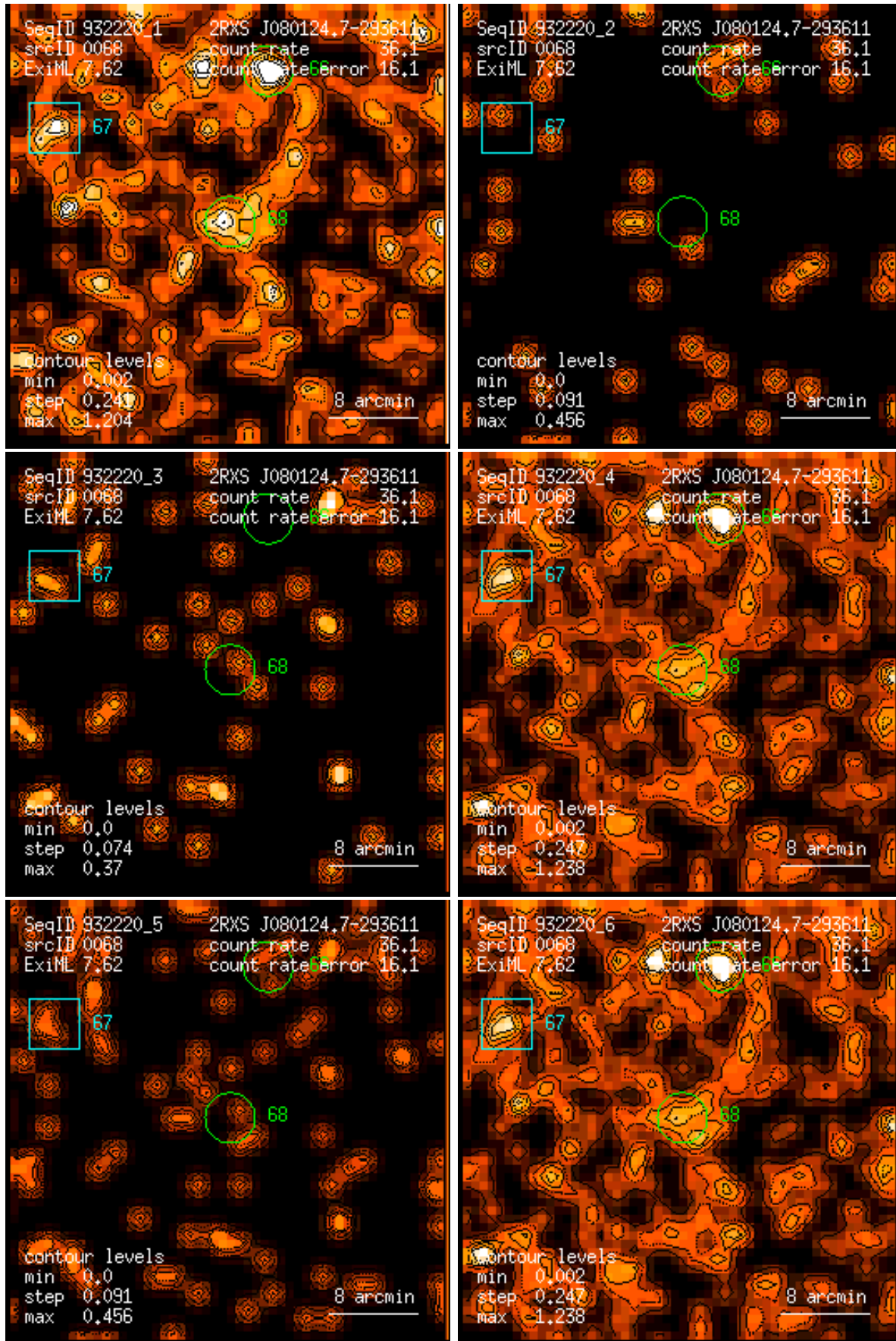
Figure 68: RASS 932220: detection 0068: band rate images, Gaussian filter: (1) PSPC channels 11 – 41, (2) 52 – 90, (3) 91 – 201, (4) 11 – 235, (5) 52 – 201, (6) 11 – 201. Broad band rates in counts/ks. Band rate contour levels in counts/ks/arcmin 2 .
