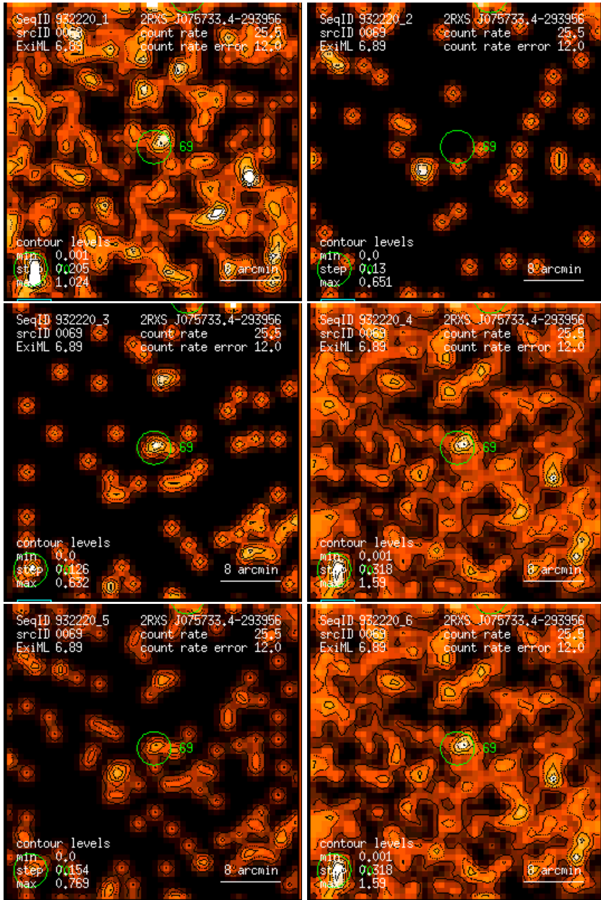
Figure 69: RASS 932220: detection 0069: band rate images, Gaussian filter: (1) PSPC channels 11 – 41, (2) 52 – 90, (3) 91 – 201, (4) 11 – 235, (5) 52 – 201, (6) 11 – 201. Broad band rates in counts/ks. Band rate contour levels in counts/ks/arcmin 2 .
