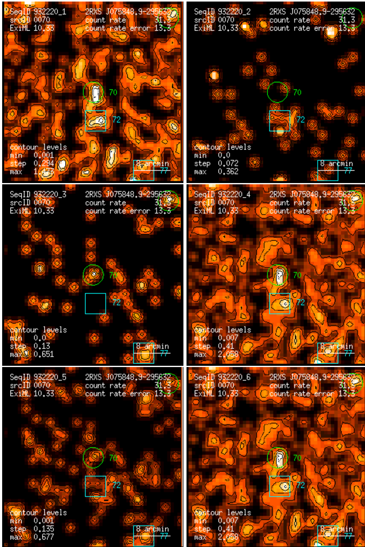
Figure 70: RASS 932220: detection 0070: band rate images, Gaussian filter: (1) PSPC channels 11 – 41, (2) 52 – 90, (3) 91 – 201, (4) 11 – 235, (5) 52 – 201, (6) 11 – 201. Broad band rates in counts/ks. Band rate contour levels in counts/ks/arcmin 2 .
