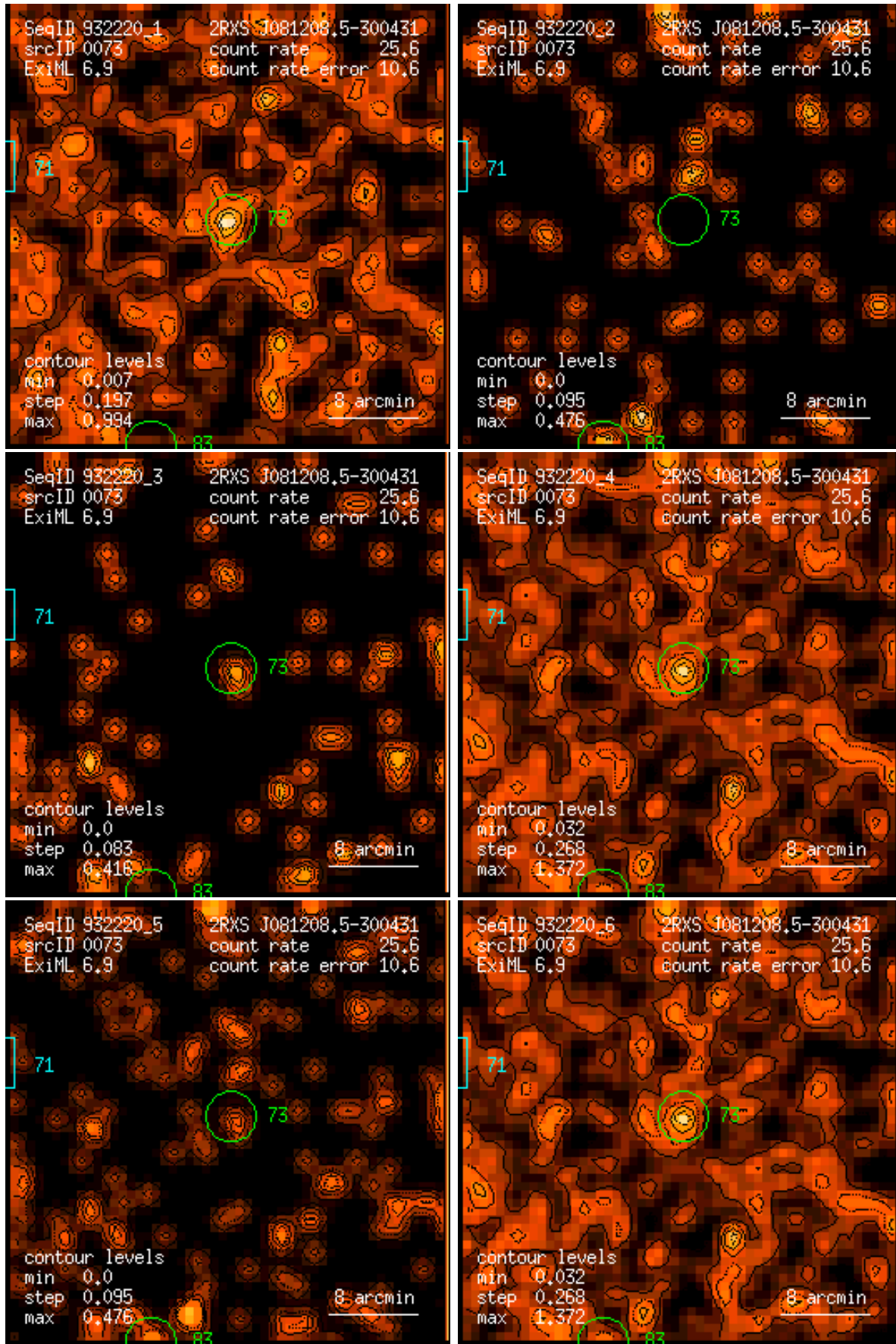
Figure 73: RASS 932220: detection 0073: band rate images, Gaussian filter: (1) PSPC channels 11 – 41, (2) 52 – 90, (3) 91 – 201, (4) 11 – 235, (5) 52 – 201, (6) 11 – 201. Broad band rates in counts/ks. Band rate contour levels in counts/ks/arcmin 2 .
