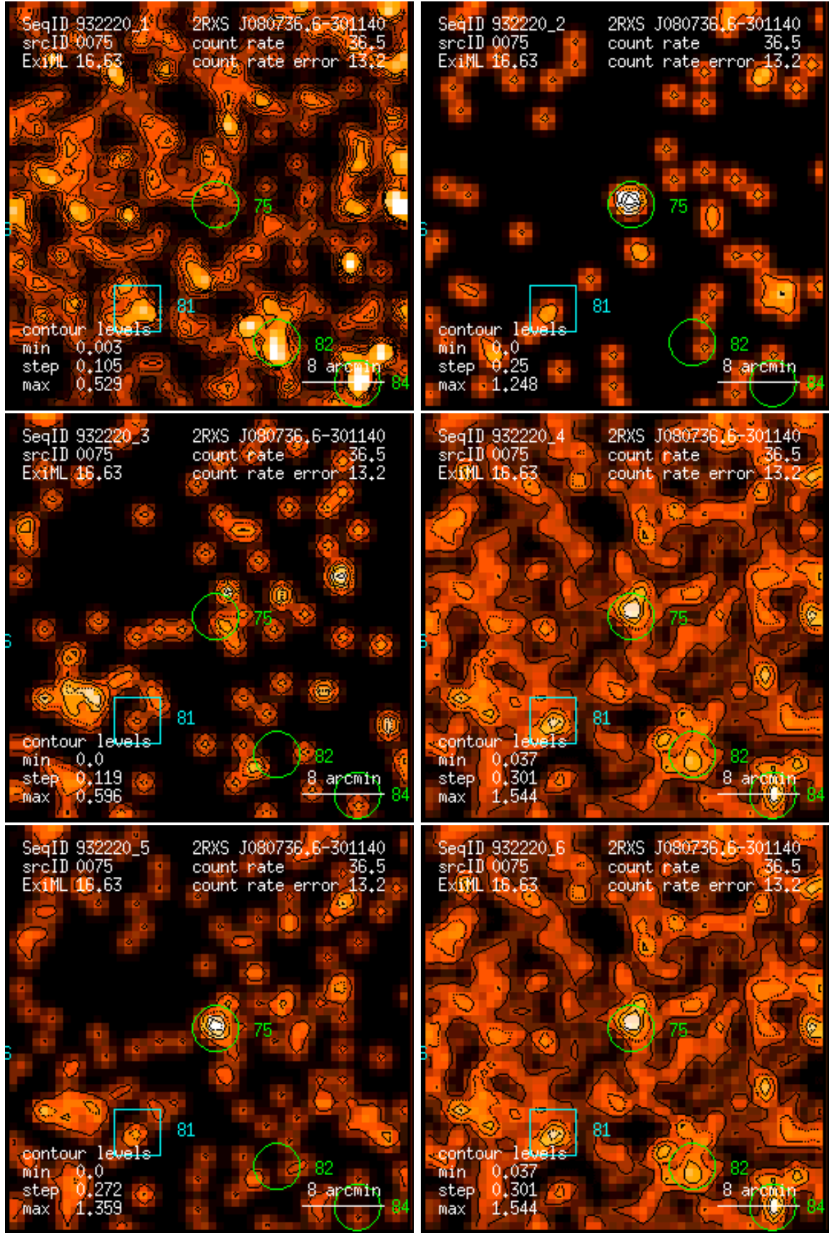
Figure 75: RASS 932220: detection 0075: band rate images, Gaussian filter: (1) PSPC channels 11 – 41, (2) 52 – 90, (3) 91 – 201, (4) 11 – 235, (5) 52 – 201, (6) 11 – 201. Broad band rates in counts/ks. Band rate contour levels in counts/ks/arcmin 2 .
