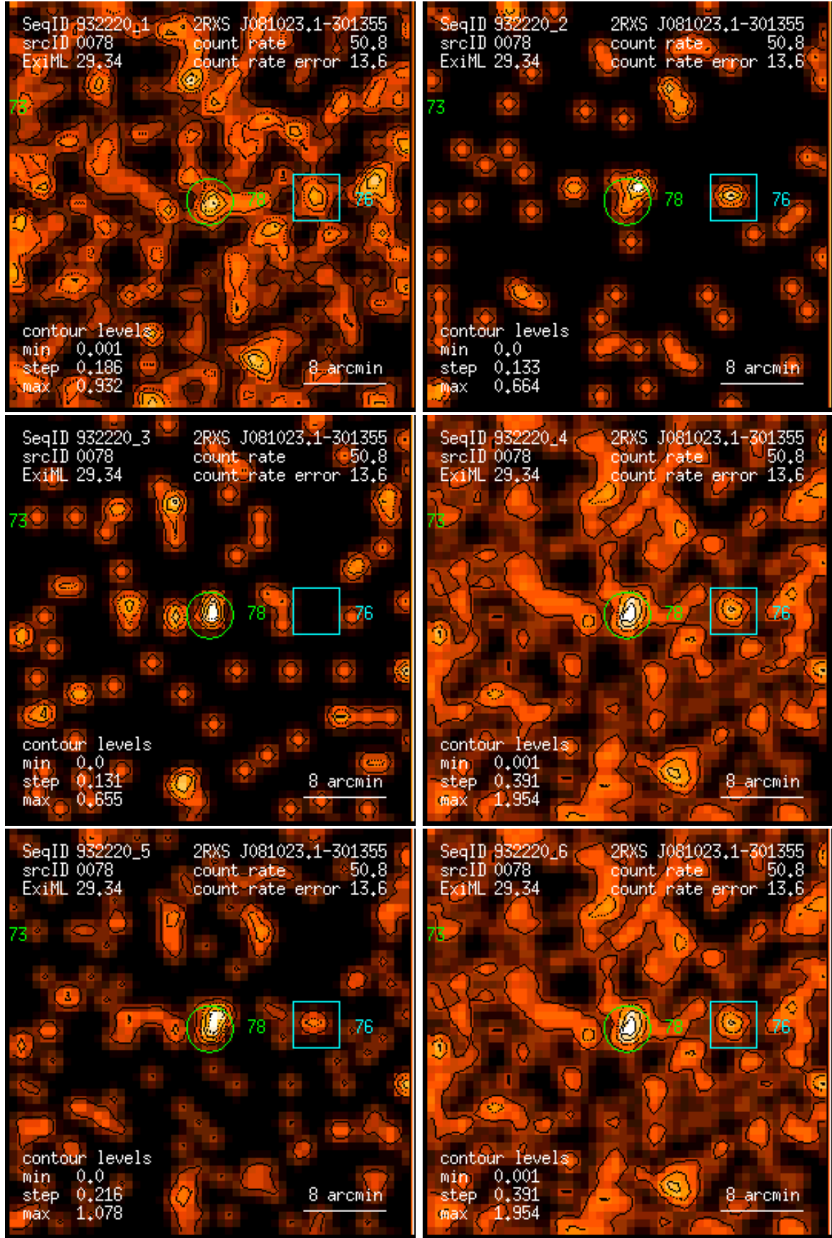
Figure 78: RASS 932220: detection 0078: band rate images, Gaussian filter: (1) PSPC channels 11 – 41, (2) 52 – 90, (3) 91 – 201, (4) 11 – 235, (5) 52 – 201, (6) 11 – 201. Broad band rates in counts/ks. Band rate contour levels in counts/ks/arcmin 2 .
