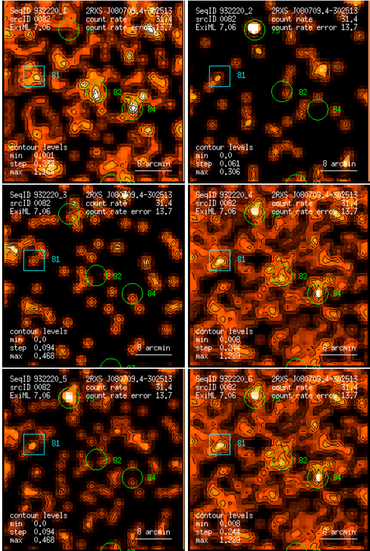
Figure 82: RASS 932220: detection 0082: band rate images, Gaussian filter: (1) PSPC channels 11 – 41, (2) 52 – 90, (3) 91 – 201, (4) 11 – 235, (5) 52 – 201, (6) 11 – 201. Broad band rates in counts/ks. Band rate contour levels in counts/ks/arcmin 2 .
