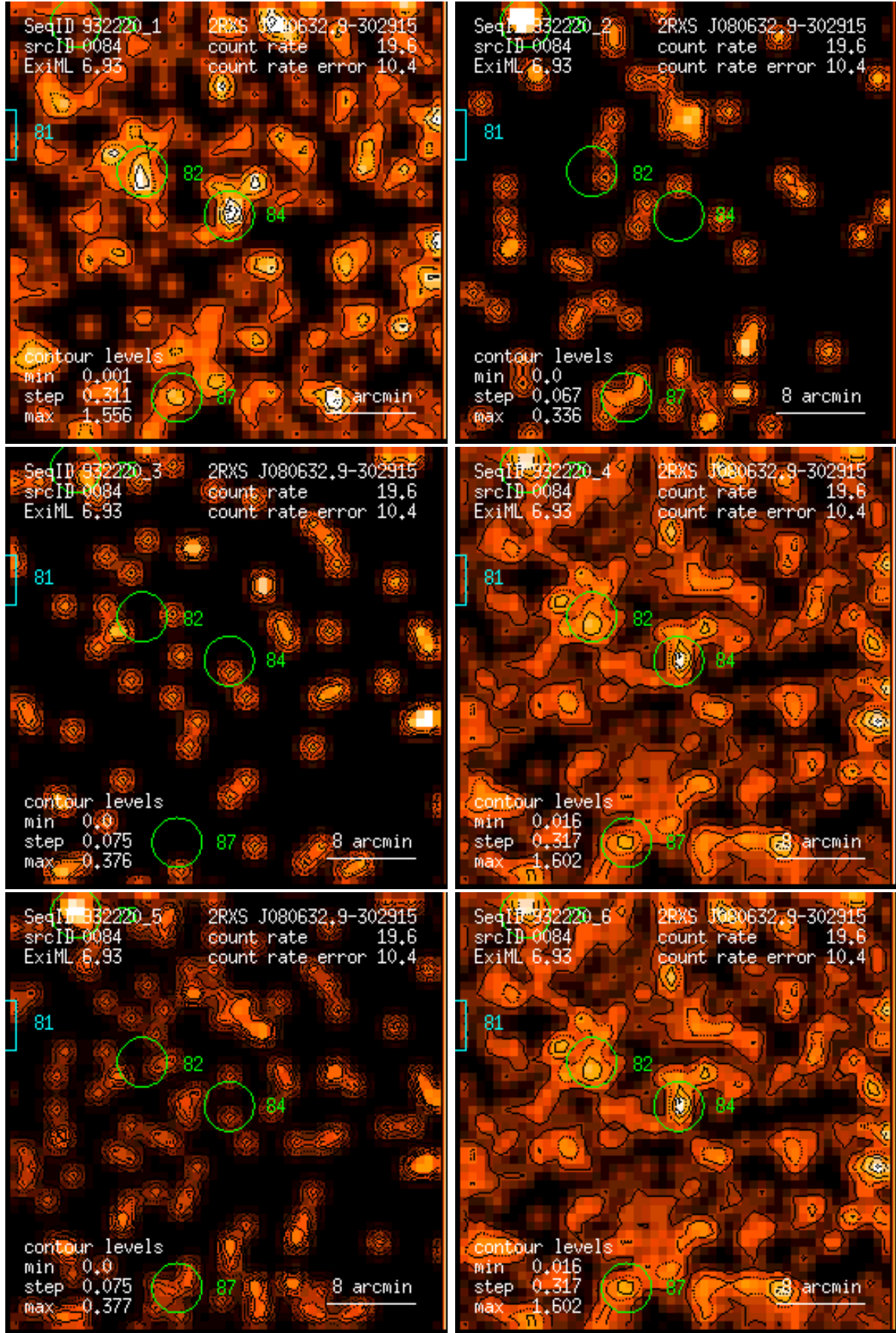
Figure 84: RASS 932220: detection 0084: band rate images, Gaussian filter: (1) PSPC channels 11 – 41, (2) 52 – 90, (3) 91 – 201, (4) 11 – 235, (5) 52 – 201, (6) 11 – 201. Broad band rates in counts/ks. Band rate contour levels in counts/ks/arcmin 2 .
