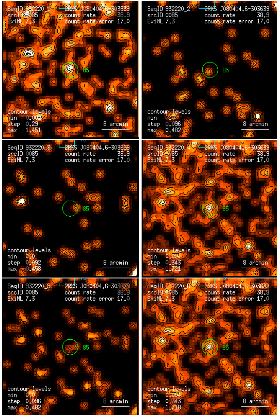
Figure 85: RASS 932220: detection 0085: band rate images, Gaussian filter: (1) PSPC channels 11 – 41, (2) 52 – 90, (3) 91 – 201, (4) 11 – 235, (5) 52 – 201, (6) 11 – 201. Broad band rates in counts/ks. Band rate contour levels in counts/ks/arcmin 2 .
