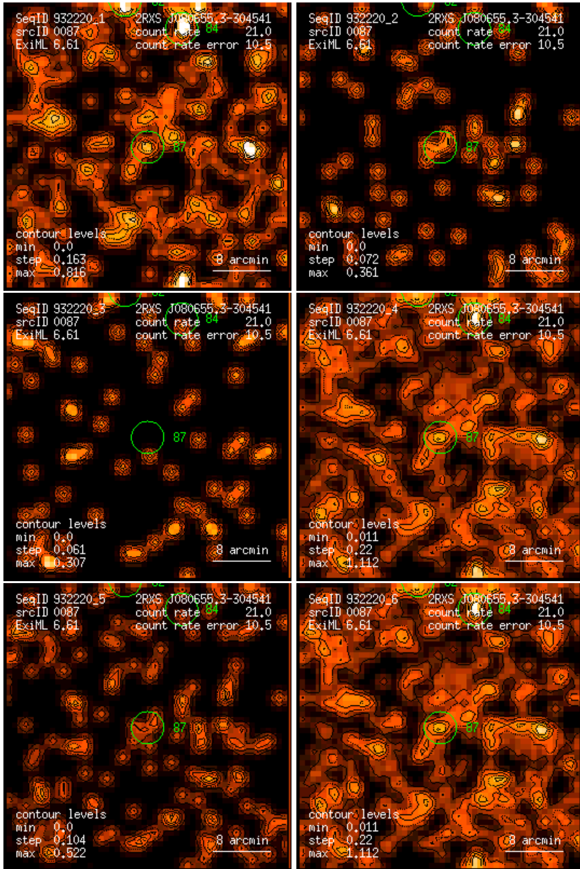
Figure 87: RASS 932220: detection 0087: band rate images, Gaussian filter: (1) PSPC channels 11 – 41, (2) 52 – 90, (3) 91 – 201, (4) 11 – 235, (5) 52 – 201, (6) 11 – 201. Broad band rates in counts/ks. Band rate contour levels in counts/ks/arcmin 2 .
