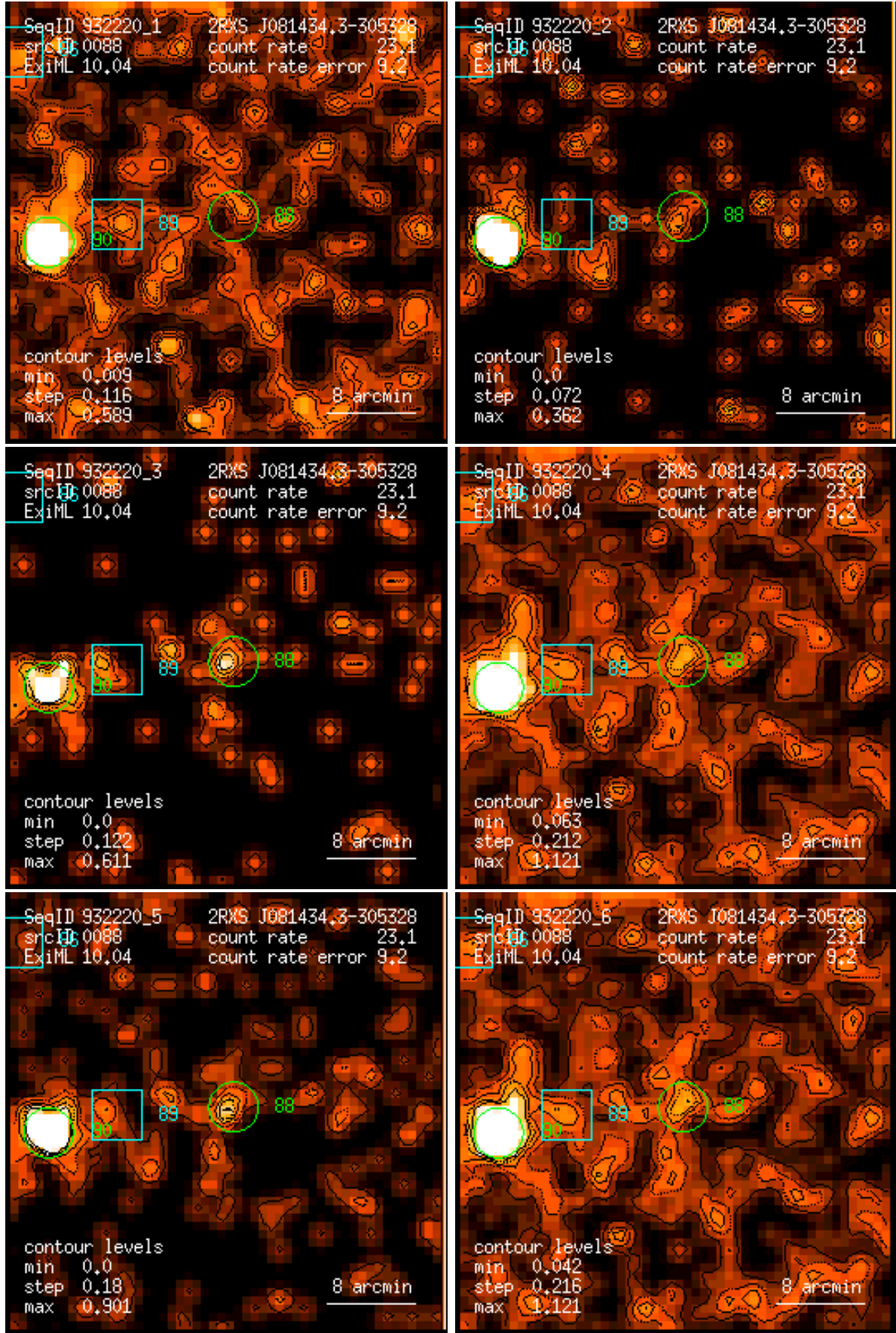
Figure 88: RASS 932220: detection 0088: band rate images, Gaussian filter: (1) PSPC channels 11 – 41, (2) 52 – 90, (3) 91 – 201, (4) 11 – 235, (5) 52 – 201, (6) 11 – 201. Broad band rates in counts/ks. Band rate contour levels in counts/ks/arcmin 2 .
