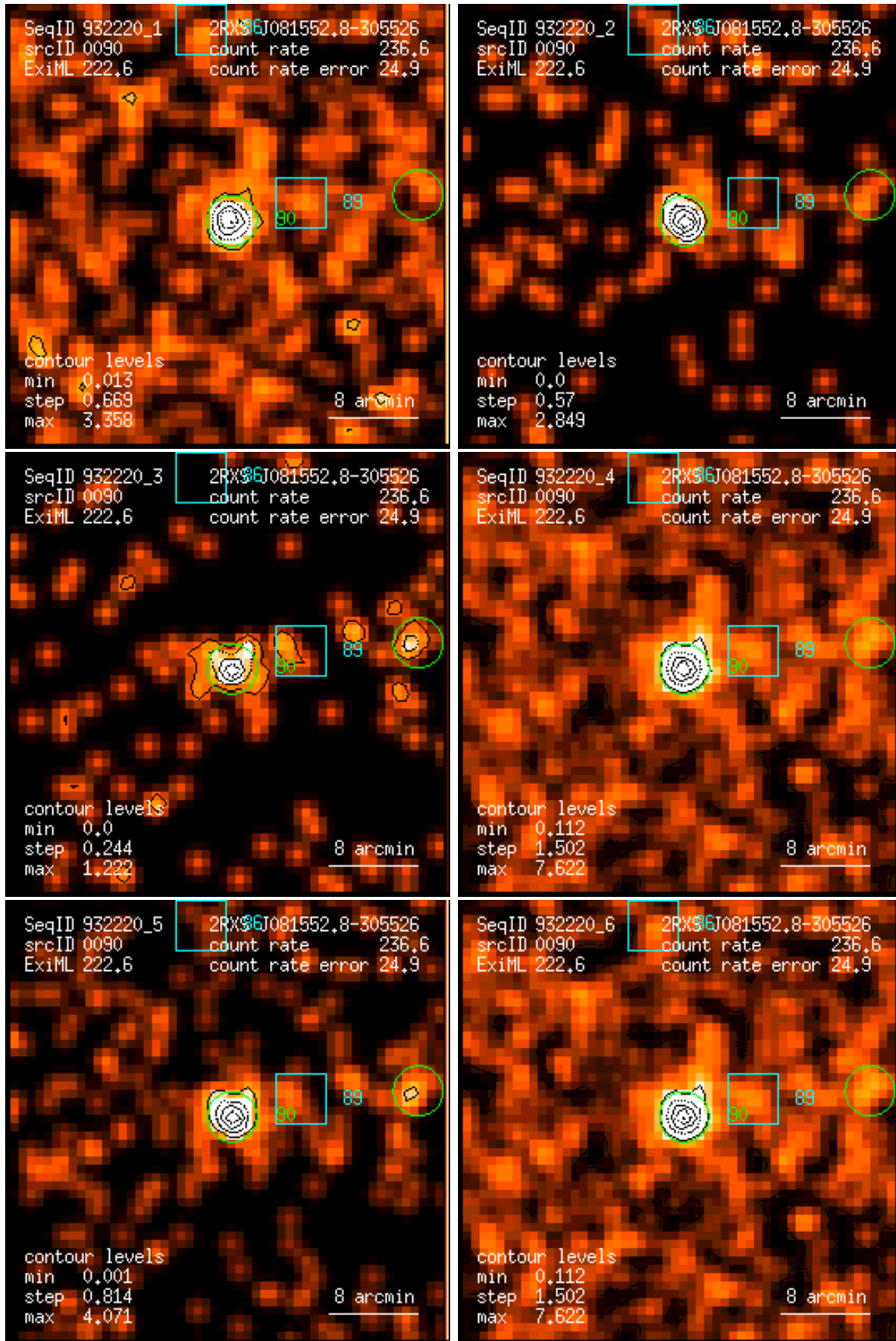
Figure 90: RASS 932220: detection 0090: band rate images, Gaussian filter: (1) PSPC channels 11 – 41, (2) 52 – 90, (3) 91 – 201, (4) 11 – 235, (5) 52 – 201, (6) 11 – 201. Broad band rates in counts/ks. Band rate contour levels in counts/ks/arcmin 2 .
