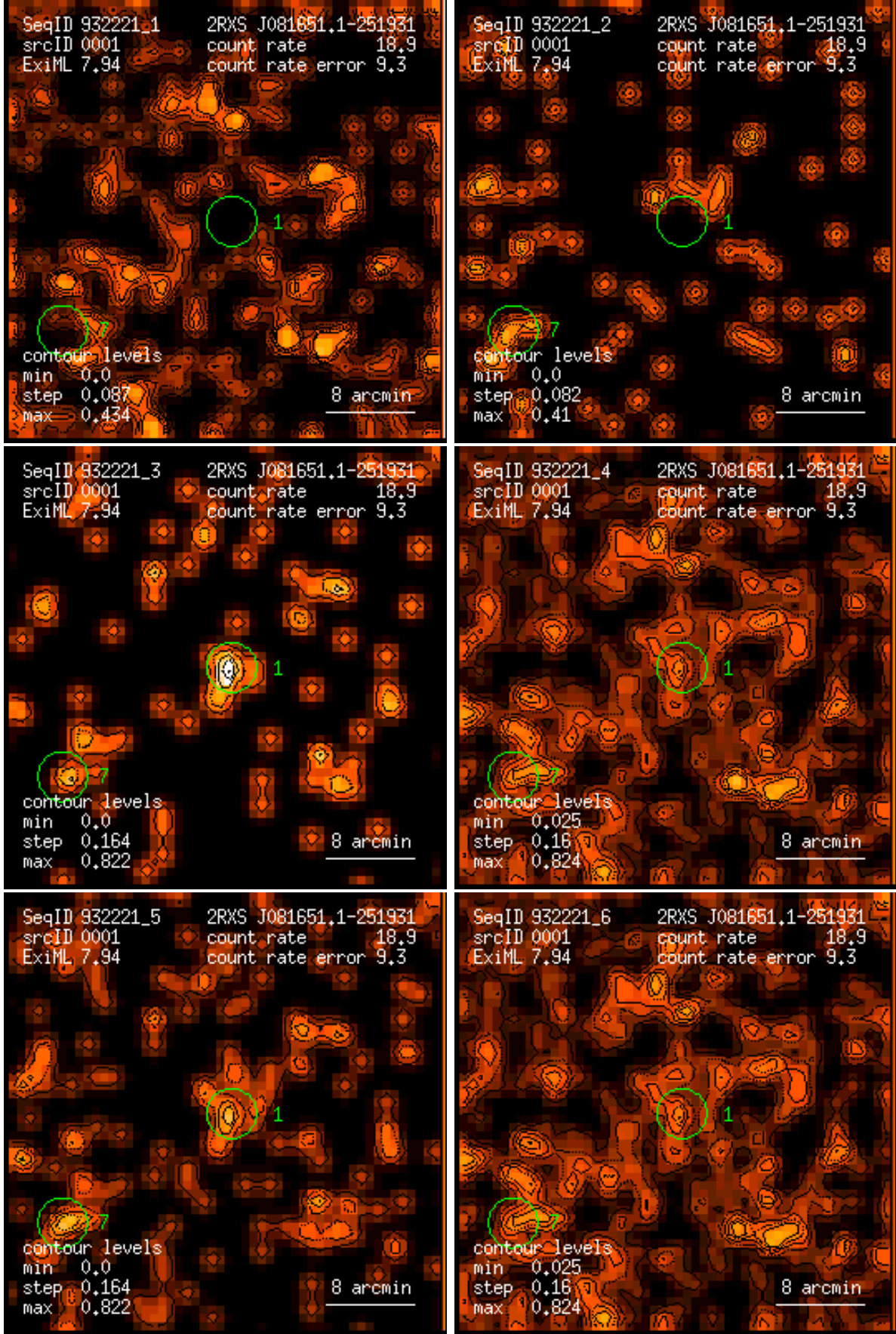
Figure 1: RASS 932221: detection 0001: band rate images, Gaussian filter: (1) PSPC channels 11 – 41, (2) 52 – 90, (3) 91 – 201, (4) 11 – 235, (5) 52 – 201, (6) 11 – 201. Broad band rates in counts/ks. Band rate contour levels in counts/ks/arcmin 2 .
