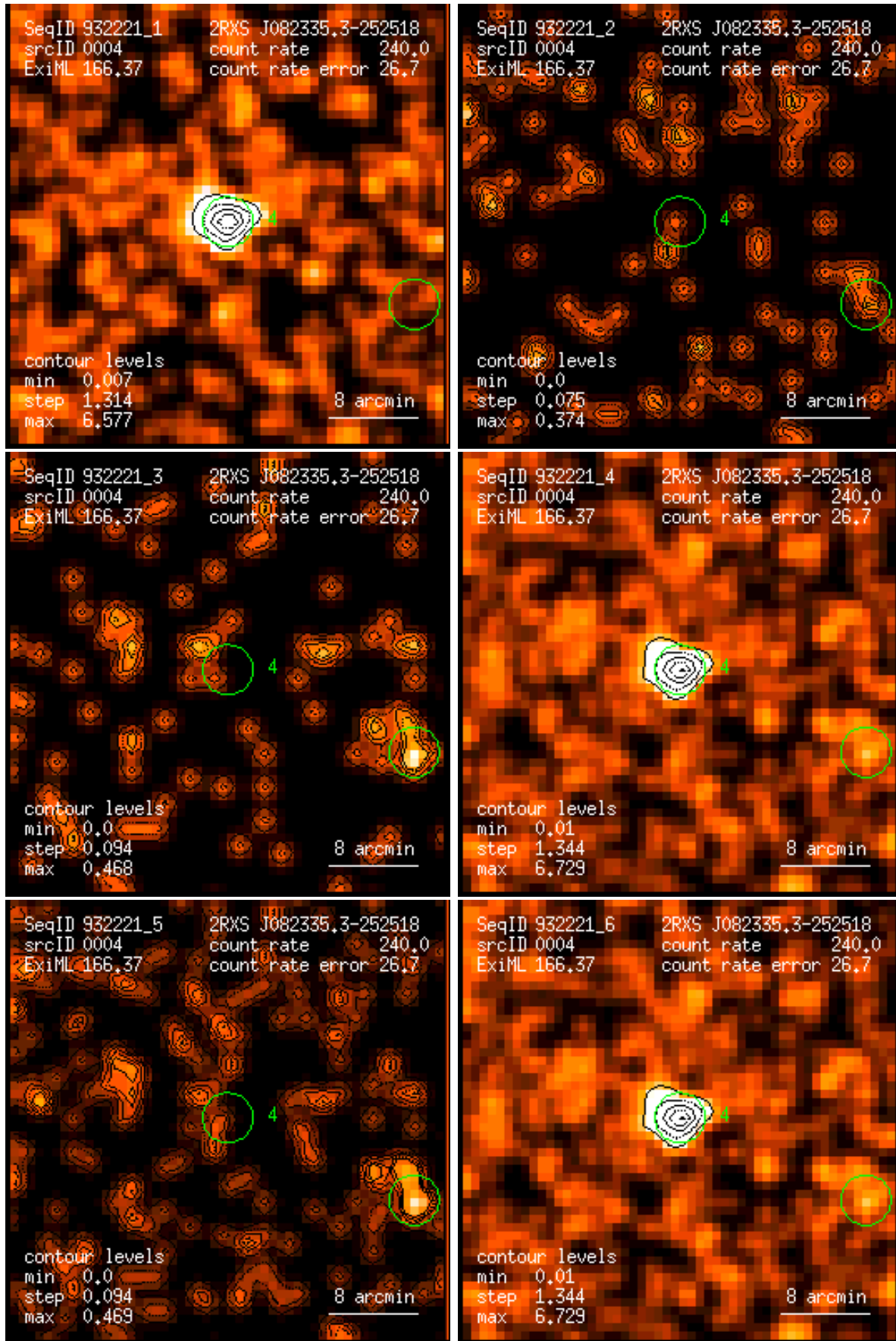
Figure 4: RASS 932221: detection 0004: band rate images, Gaussian filter: (1) PSPC channels 11 – 41, (2) 52 – 90, (3) 91 – 201, (4) 11 – 235, (5) 52 – 201, (6) 11 – 201. Broad band rates in counts/ks. Band rate contour levels in counts/ks/arcmin 2 .
