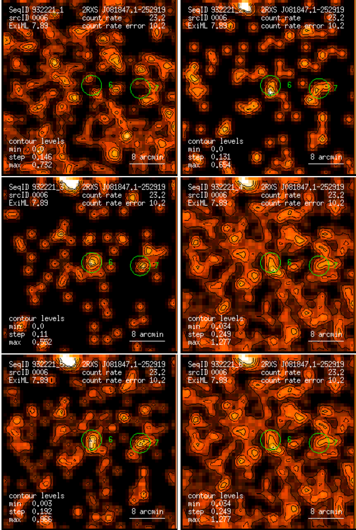
Figure 6: RASS 932221: detection 0006: band rate images, Gaussian filter: (1) PSPC channels 11 – 41, (2) 52 – 90, (3) 91 – 201, (4) 11 – 235, (5) 52 – 201, (6) 11 – 201. Broad band rates in counts/ks. Band rate contour levels in counts/ks/arcmin 2 .
