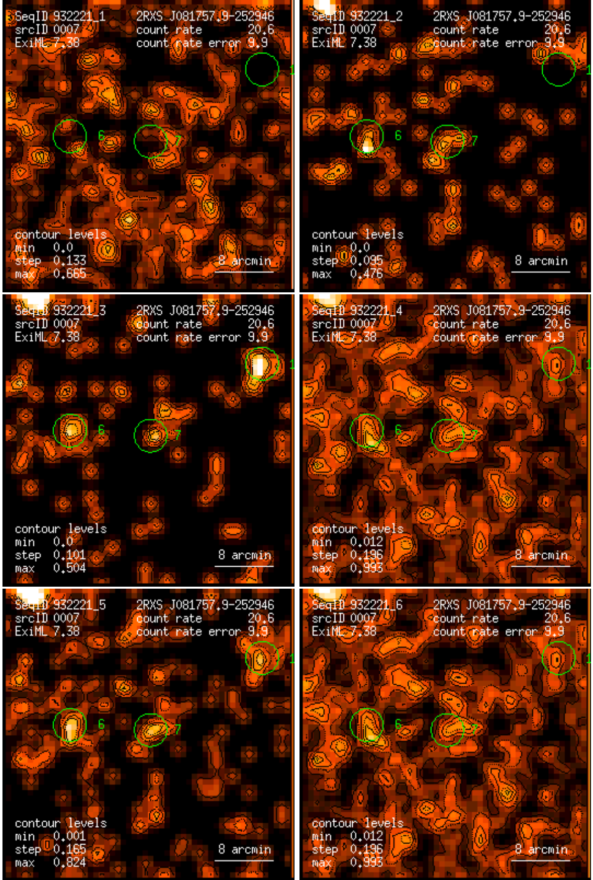
Figure 7: RASS 932221: detection 0007: band rate images, Gaussian filter: (1) PSPC channels 11 – 41, (2) 52 – 90, (3) 91 – 201, (4) 11 – 235, (5) 52 – 201, (6) 11 – 201. Broad band rates in counts/ks. Band rate contour levels in counts/ks/arcmin 2 .
