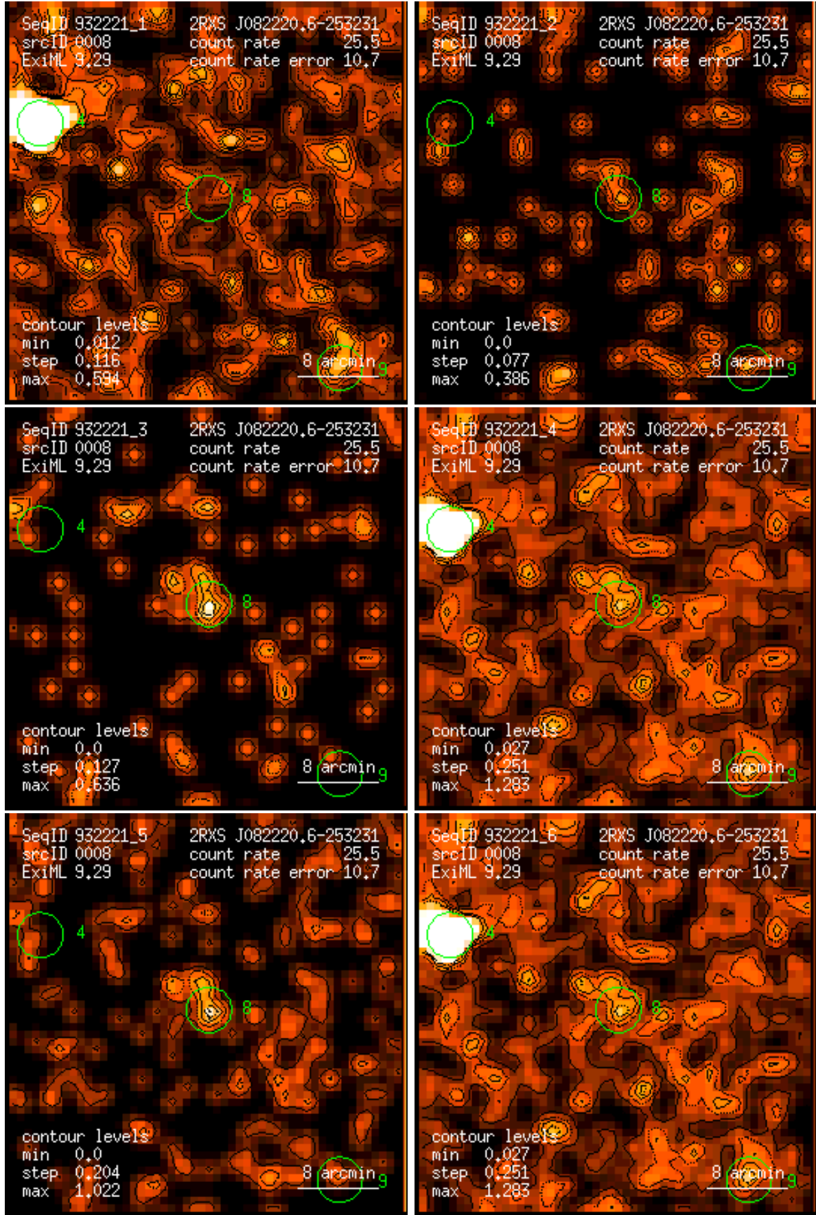
Figure 8: RASS 932221: detection 0008: band rate images, Gaussian filter: (1) PSPC channels 11 – 41, (2) 52 – 90, (3) 91 – 201, (4) 11 – 235, (5) 52 – 201, (6) 11 – 201. Broad band rates in counts/ks. Band rate contour levels in counts/ks/arcmin 2 .
