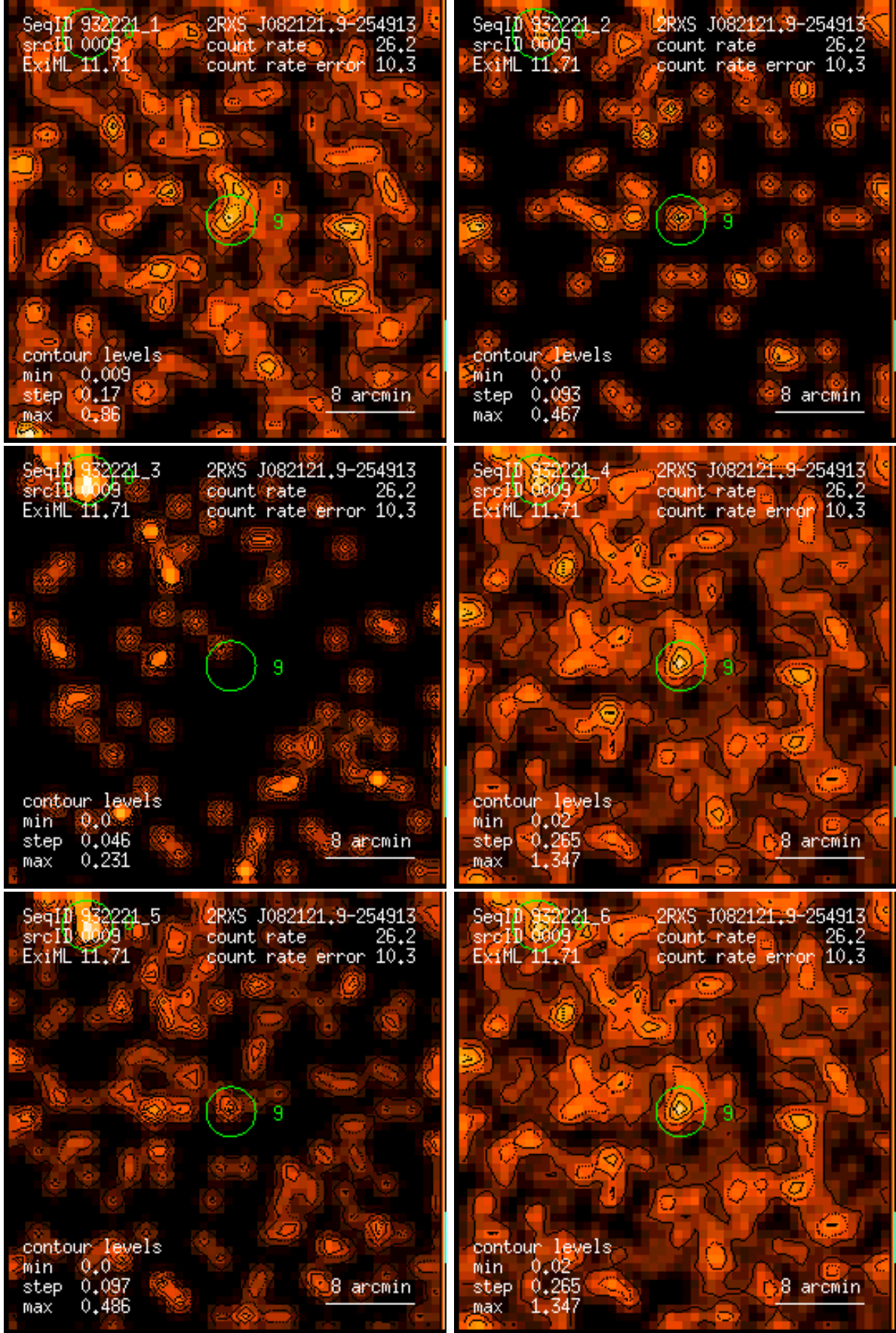
Figure 9: RASS 932221: detection 0009: band rate images, Gaussian filter: (1) PSPC channels 11 – 41, (2) 52 – 90, (3) 91 – 201, (4) 11 – 235, (5) 52 – 201, (6) 11 – 201. Broad band rates in counts/ks. Band rate contour levels in counts/ks/arcmin 2 .
