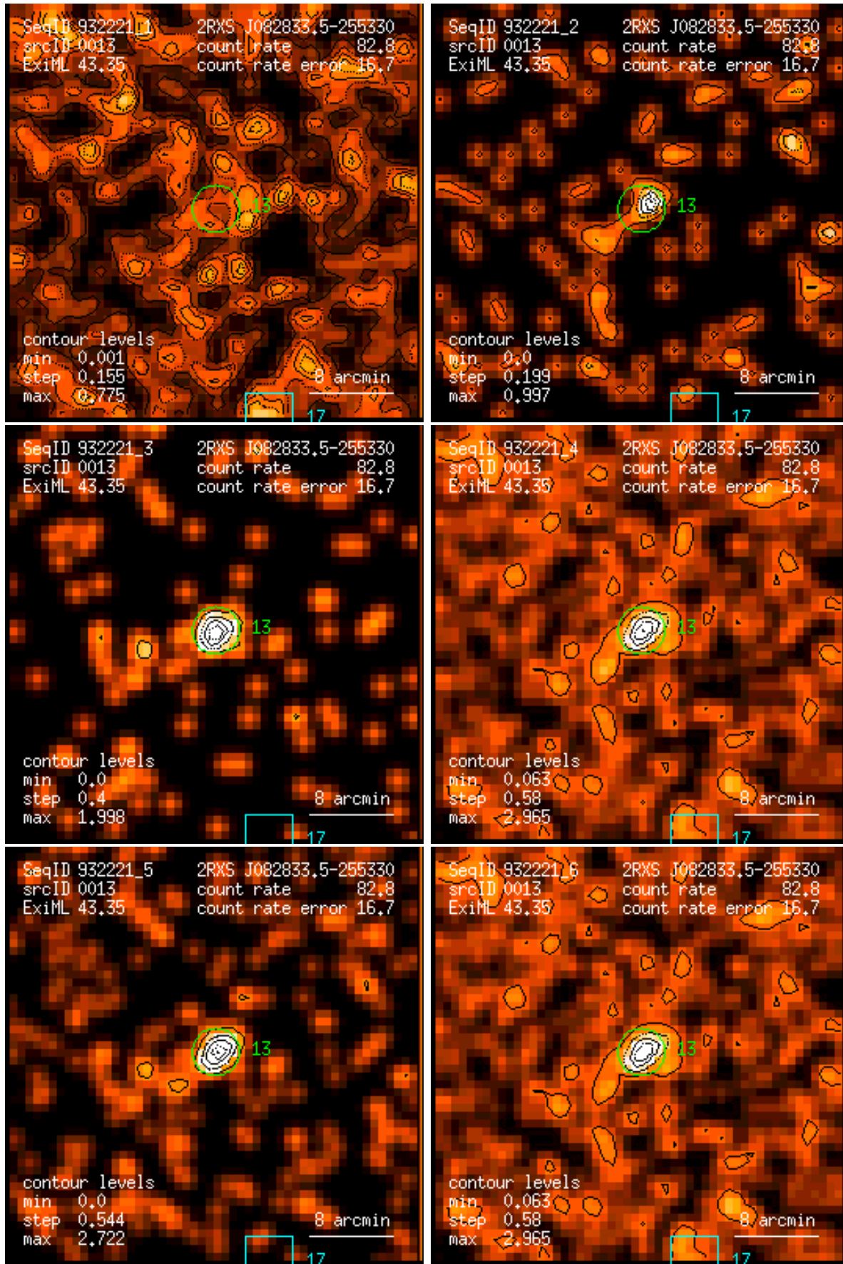
Figure 13: RASS 932221: detection 0013: band rate images, Gaussian filter: (1) PSPC channels 11 – 41, (2) 52 – 90, (3) 91 – 201, (4) 11 – 235, (5) 52 – 201, (6) 11 – 201. Broad band rates in counts/ks. Band rate contour levels in counts/ks/arcmin 2 .
