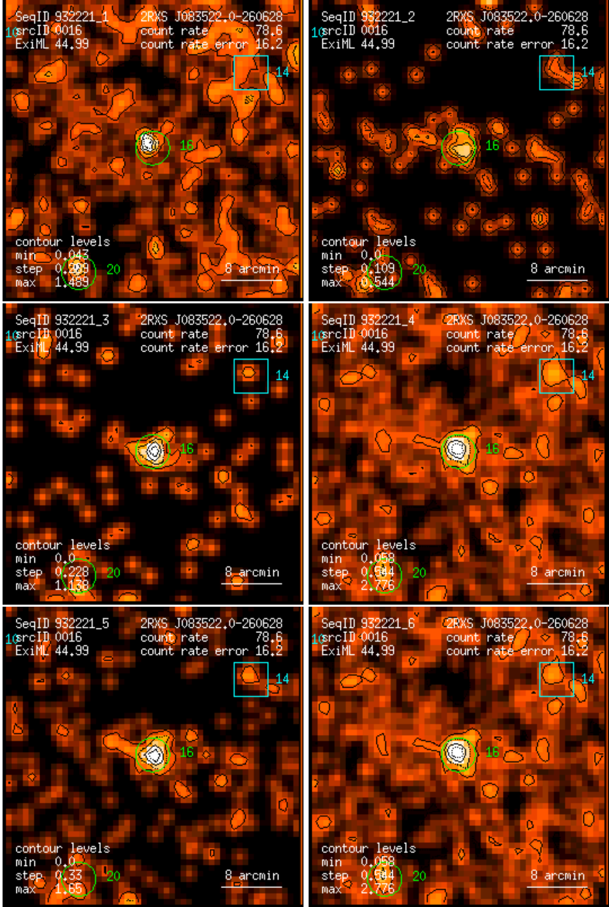
Figure 16: RASS 932221: detection 0016: band rate images, Gaussian filter: (1) PSPC channels 11 – 41, (2) 52 – 90, (3) 91 – 201, (4) 11 – 235, (5) 52 – 201, (6) 11 – 201. Broad band rates in counts/ks. Band rate contour levels in counts/ks/arcmin 2 .
