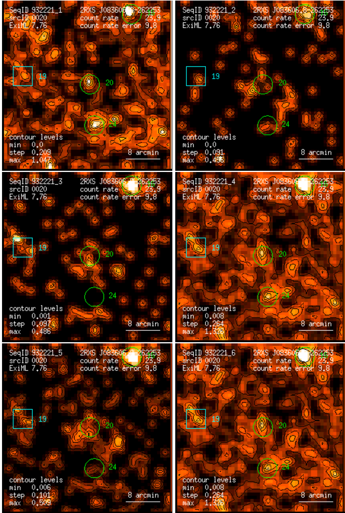
Figure 20: RASS 932221: detection 0020: band rate images, Gaussian filter: (1) PSPC channels 11 – 41, (2) 52 – 90, (3) 91 – 201, (4) 11 – 235, (5) 52 – 201, (6) 11 – 201. Broad band rates in counts/ks. Band rate contour levels in counts/ks/arcmin 2 .
