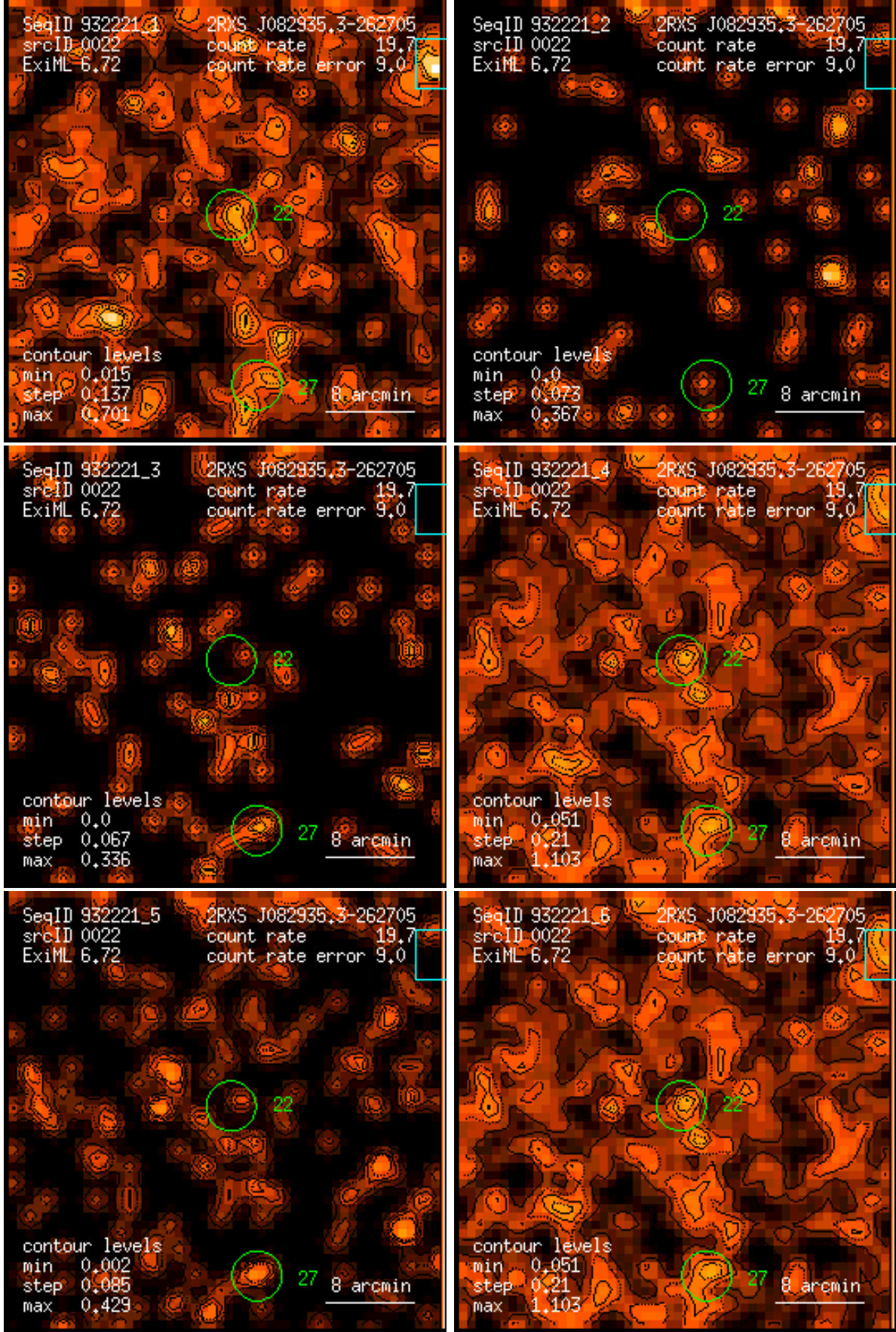
Figure 22: RASS 932221: detection 0022: band rate images, Gaussian filter: (1) PSPC channels 11 – 41, (2) 52 – 90, (3) 91 – 201, (4) 11 – 235, (5) 52 – 201, (6) 11 – 201. Broad band rates in counts/ks. Band rate contour levels in counts/ks/arcmin 2 .
