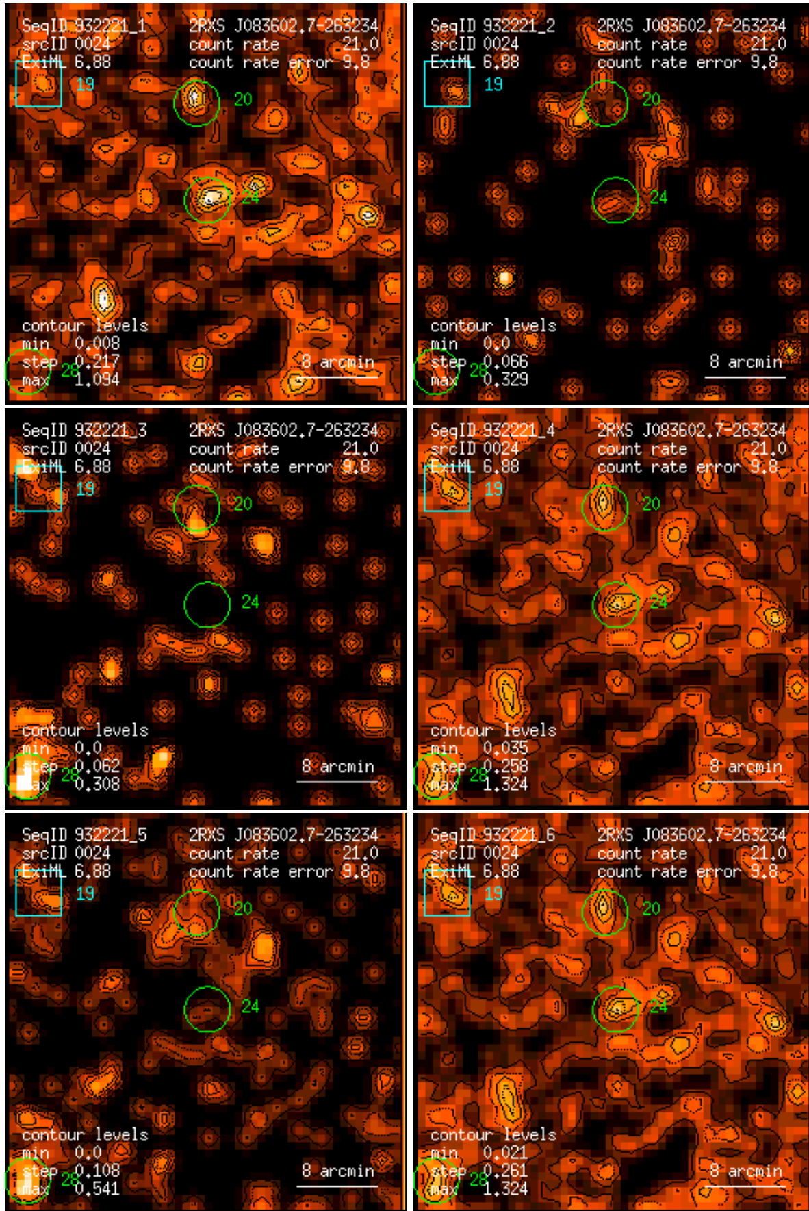
Figure 24: RASS 932221: detection 0024: band rate images, Gaussian filter: (1) PSPC channels 11 – 41, (2) 52 – 90, (3) 91 – 201, (4) 11 – 235, (5) 52 – 201, (6) 11 – 201. Broad band rates in counts/ks. Band rate contour levels in counts/ks/arcmin 2 .
