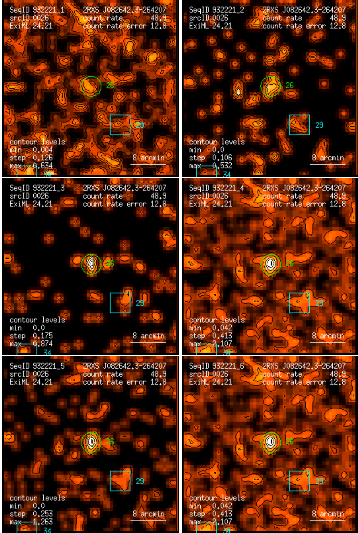
Figure 26: RASS 932221: detection 0026: band rate images, Gaussian filter: (1) PSPC channels 11 – 41, (2) 52 – 90, (3) 91 – 201, (4) 11 – 235, (5) 52 – 201, (6) 11 – 201. Broad band rates in counts/ks. Band rate contour levels in counts/ks/arcmin 2 .
