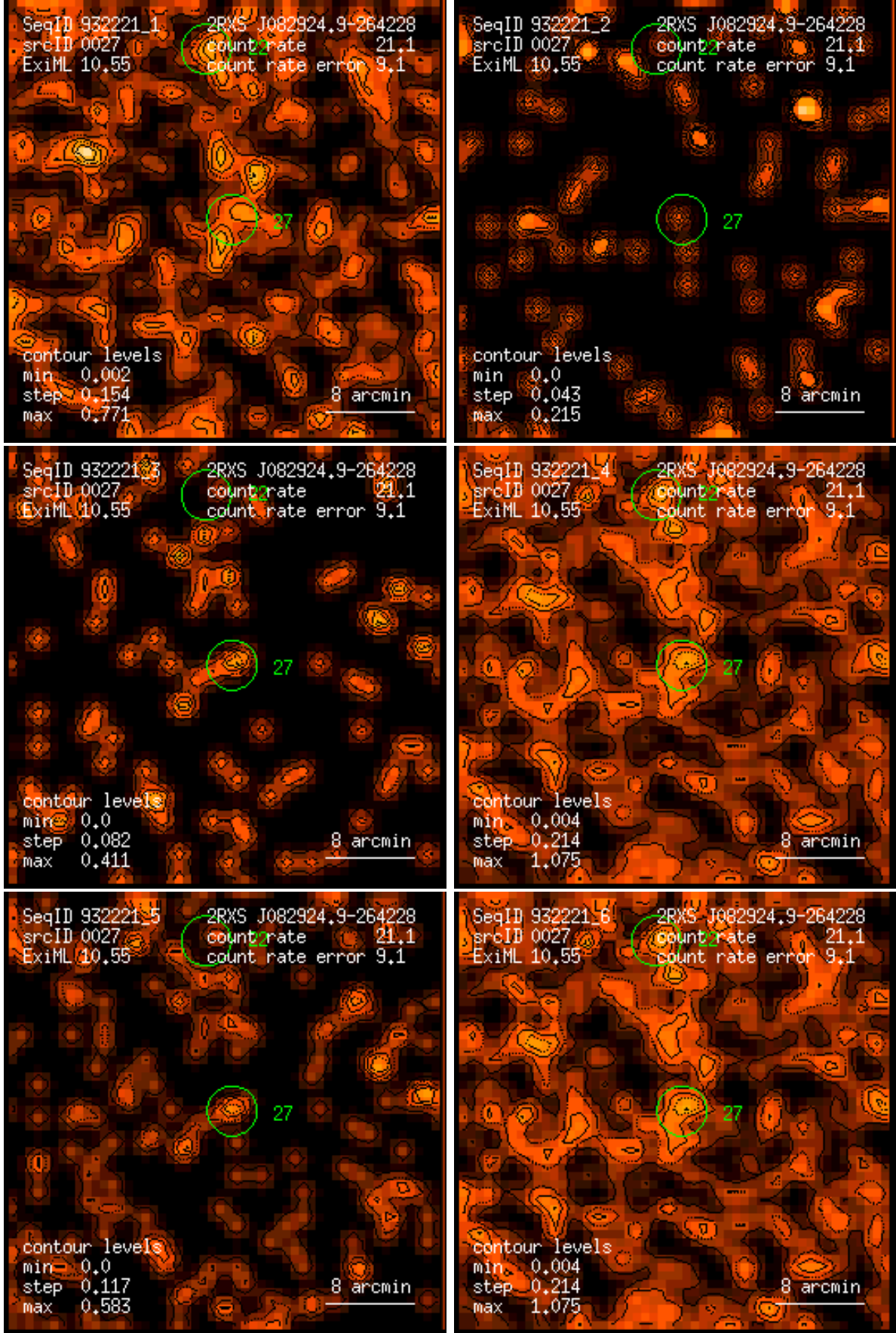
Figure 27: RASS 932221: detection 0027: band rate images, Gaussian filter: (1) PSPC channels 11 – 41, (2) 52 – 90, (3) 91 – 201, (4) 11 – 235, (5) 52 – 201, (6) 11 – 201. Broad band rates in counts/ks. Band rate contour levels in counts/ks/arcmin 2 .
