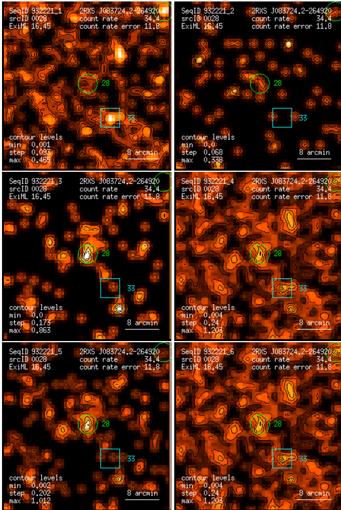
Figure 28: RASS 932221: detection 0028: band rate images, Gaussian filter: (1) PSPC channels 11 – 41, (2) 52 – 90, (3) 91 – 201, (4) 11 – 235, (5) 52 – 201, (6) 11 – 201. Broad band rates in counts/ks. Band rate contour levels in counts/ks/arcmin 2 .
