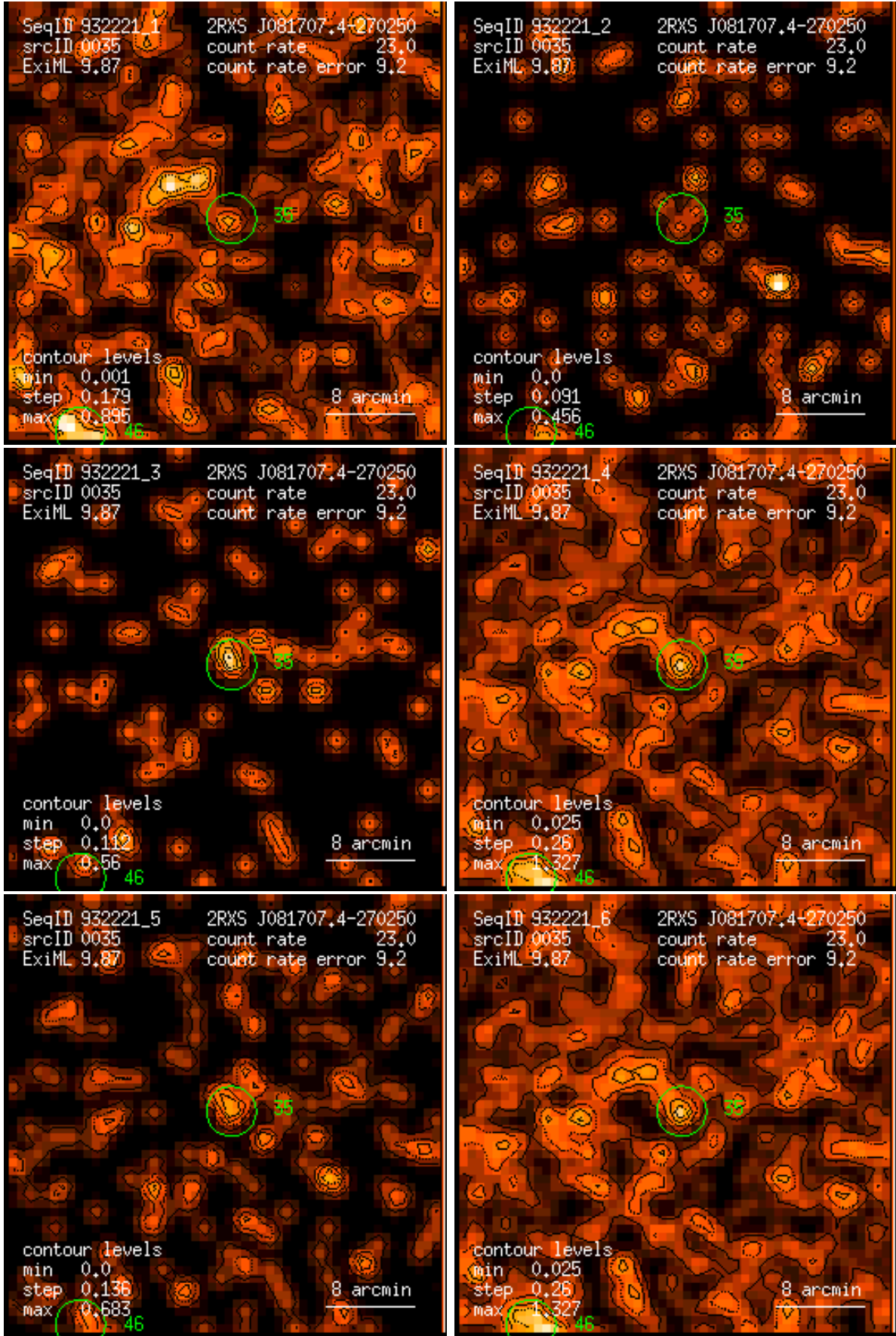
Figure 35: RASS 932221: detection 0035: band rate images, Gaussian filter: (1) PSPC channels 11 – 41, (2) 52 – 90, (3) 91 – 201, (4) 11 – 235, (5) 52 – 201, (6) 11 – 201. Broad band rates in counts/ks. Band rate contour levels in counts/ks/arcmin 2 .
