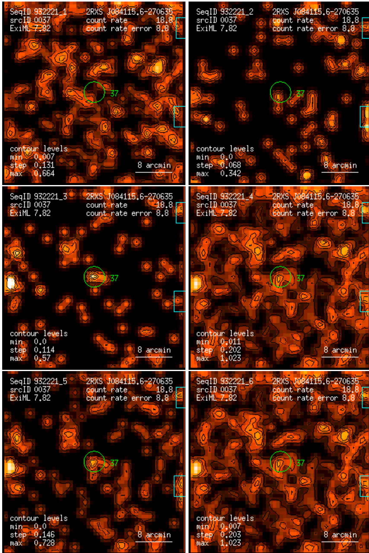
Figure 37: RASS 932221: detection 0037: band rate images, Gaussian filter: (1) PSPC channels 11 – 41, (2) 52 – 90, (3) 91 – 201, (4) 11 – 235, (5) 52 – 201, (6) 11 – 201. Broad band rates in counts/ks. Band rate contour levels in counts/ks/arcmin 2 .
