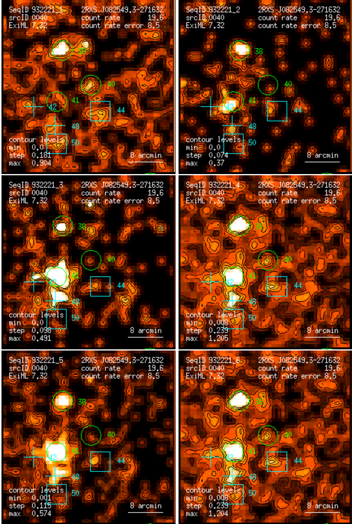
Figure 40: RASS 932221: detection 0040: band rate images, Gaussian filter: (1) PSPC channels 11 – 41, (2) 52 – 90, (3) 91 – 201, (4) 11 – 235, (5) 52 – 201, (6) 11 – 201. Broad band rates in counts/ks. Band rate contour levels in counts/ks/arcmin 2 .
