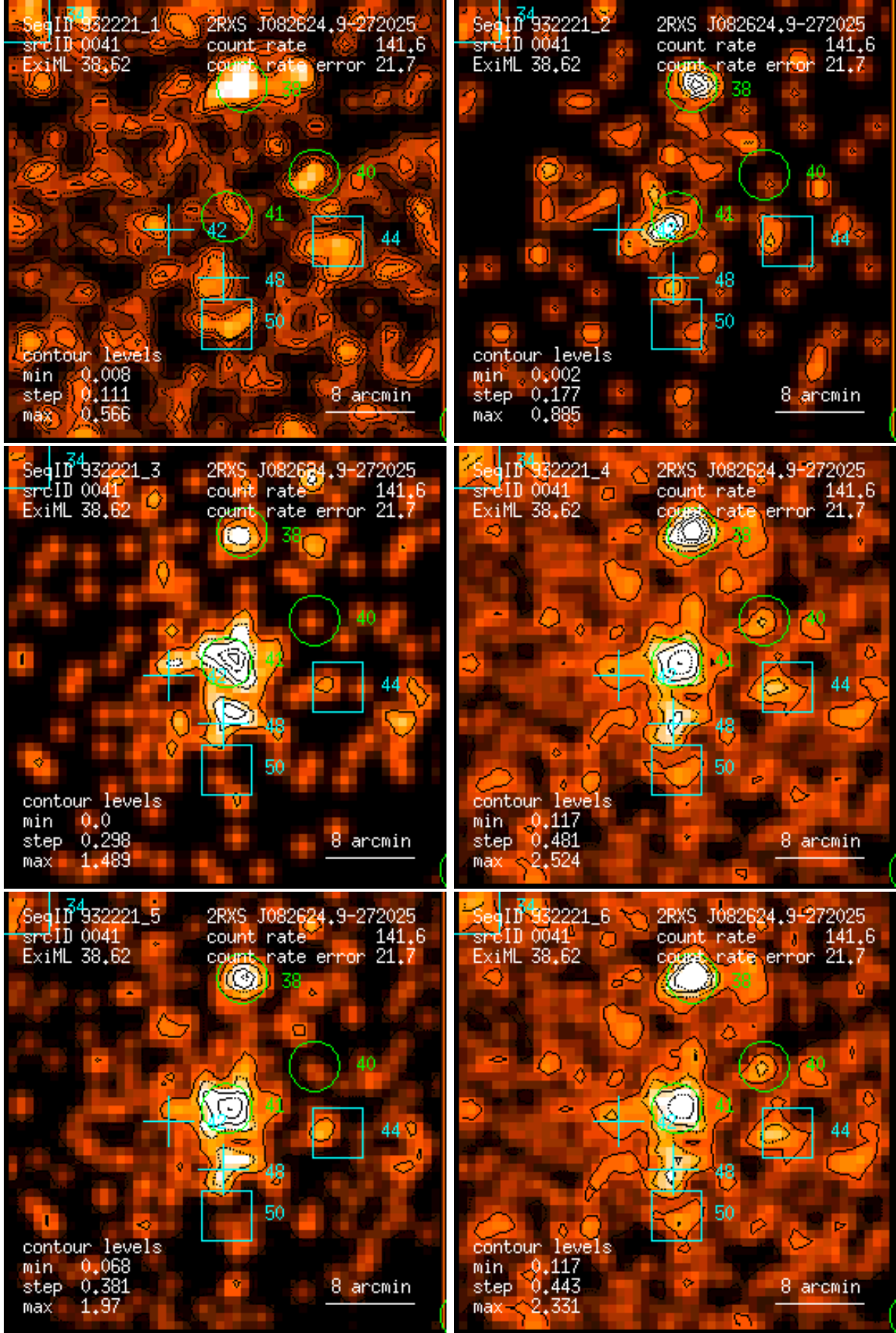
Figure 41: RASS 932221: detection 0041: band rate images, Gaussian filter: (1) PSPC channels 11 – 41, (2) 52 – 90, (3) 91 – 201, (4) 11 – 235, (5) 52 – 201, (6) 11 – 201. Broad band rates in counts/ks. Band rate contour levels in counts/ks/arcmin 2 .
