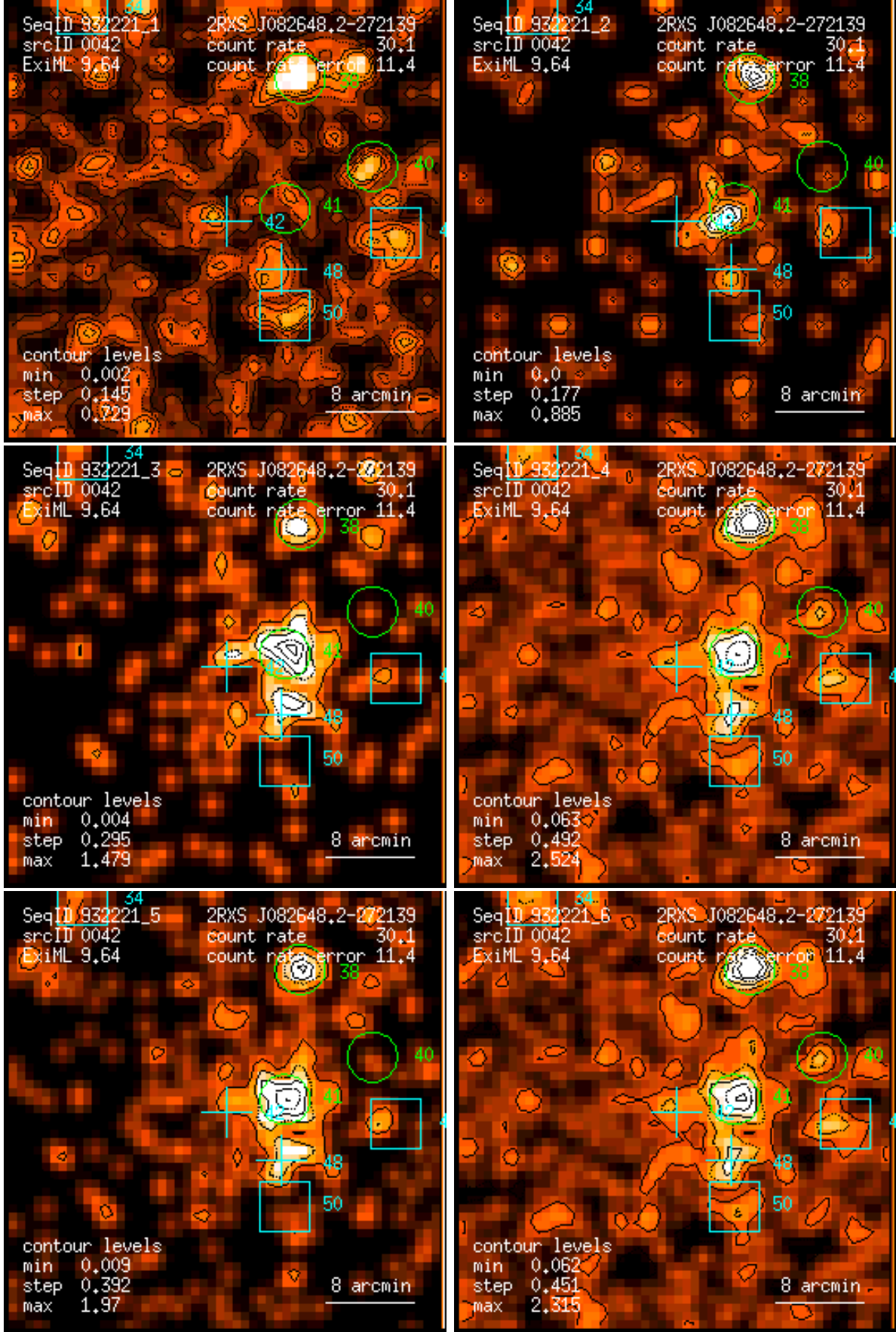
Figure 42: RASS 932221: detection 0042: band rate images, Gaussian filter: (1) PSPC channels 11 – 41, (2) 52 – 90, (3) 91 – 201, (4) 11 – 235, (5) 52 – 201, (6) 11 – 201. Broad band rates in counts/ks. Band rate contour levels in counts/ks/arcmin 2 .
