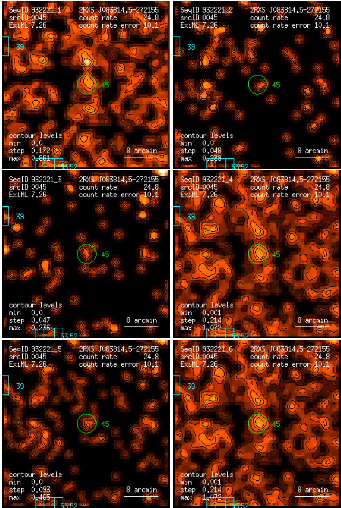
Figure 45: RASS 932221: detection 0045: band rate images, Gaussian filter: (1) PSPC channels 11 – 41, (2) 52 – 90, (3) 91 – 201, (4) 11 – 235, (5) 52 – 201, (6) 11 – 201. Broad band rates in counts/ks. Band rate contour levels in counts/ks/arcmin 2 .
