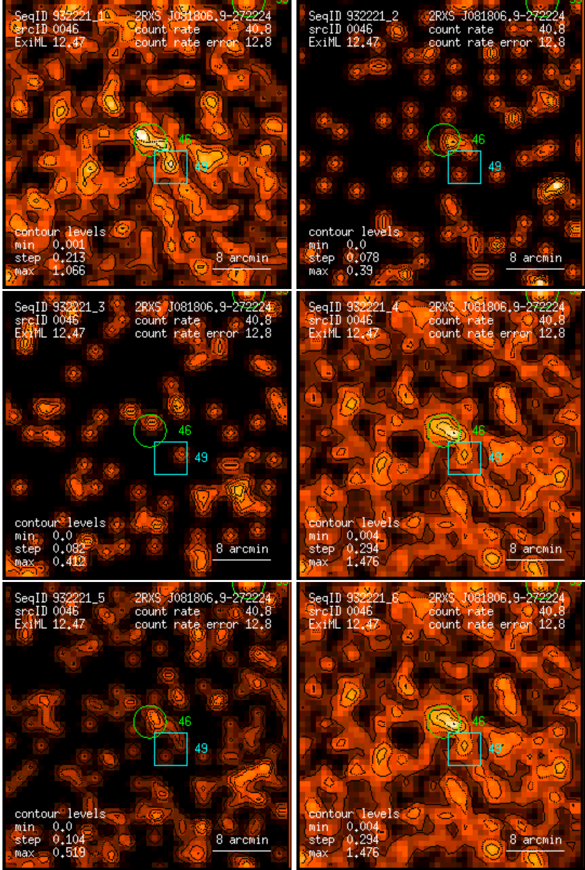
Figure 46: RASS 932221: detection 0046: band rate images, Gaussian filter: (1) PSPC channels 11 – 41, (2) 52 – 90, (3) 91 – 201, (4) 11 – 235, (5) 52 – 201, (6) 11 – 201. Broad band rates in counts/ks. Band rate contour levels in counts/ks/arcmin 2 .
