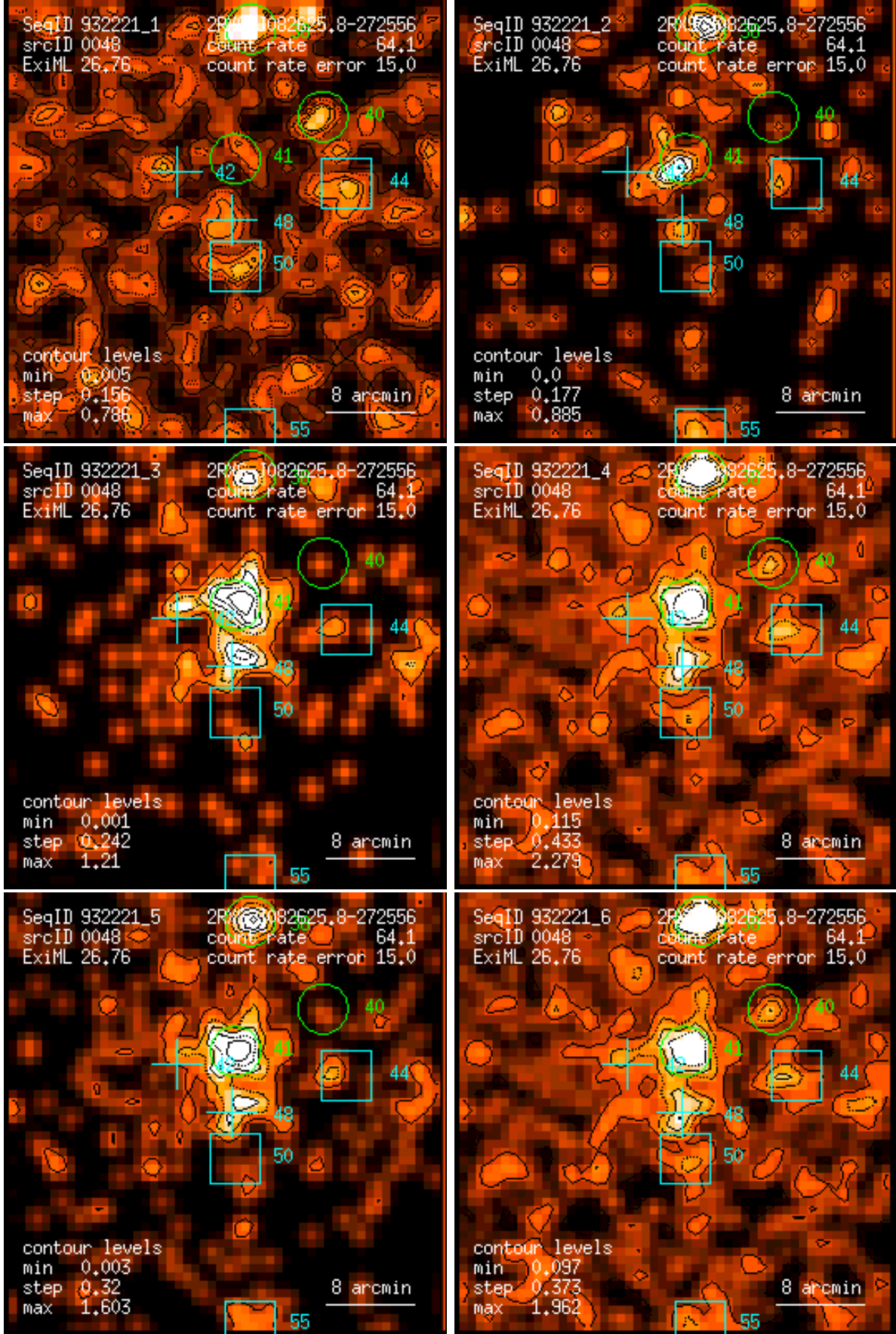
Figure 48: RASS 932221: detection 0048: band rate images, Gaussian filter: (1) PSPC channels 11 – 41, (2) 52 – 90, (3) 91 – 201, (4) 11 – 235, (5) 52 – 201, (6) 11 – 201. Broad band rates in counts/ks. Band rate contour levels in counts/ks/arcmin 2 .
